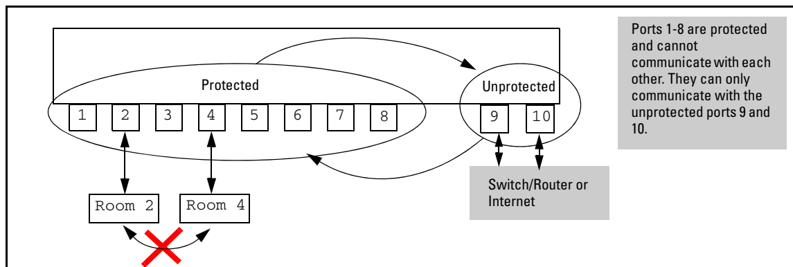
Figure 9-25. Example With Ports 1-8 Protected and Ports 9 and 10 Unprotected
