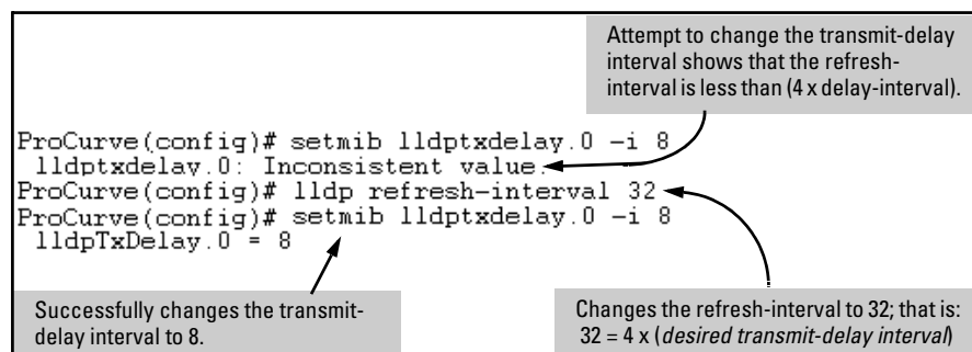
Figure 13-3. Example of Changing the Transmit-Delay Interval
