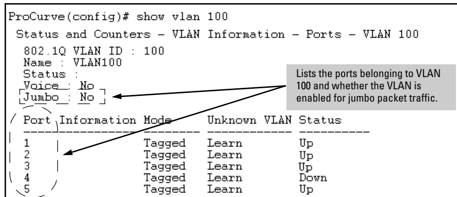
Figure 10-6. Example of Listing the Port Membership and Jumbo Status for a VLAN
