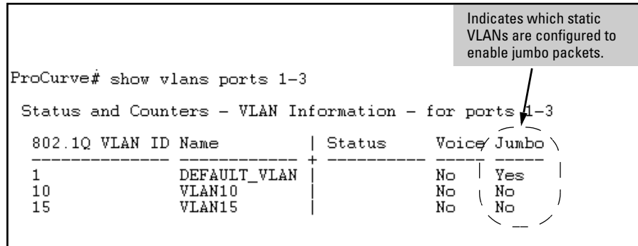
Figure 10-5. Example of Listing the VLAN Memberships for a Range of Ports
