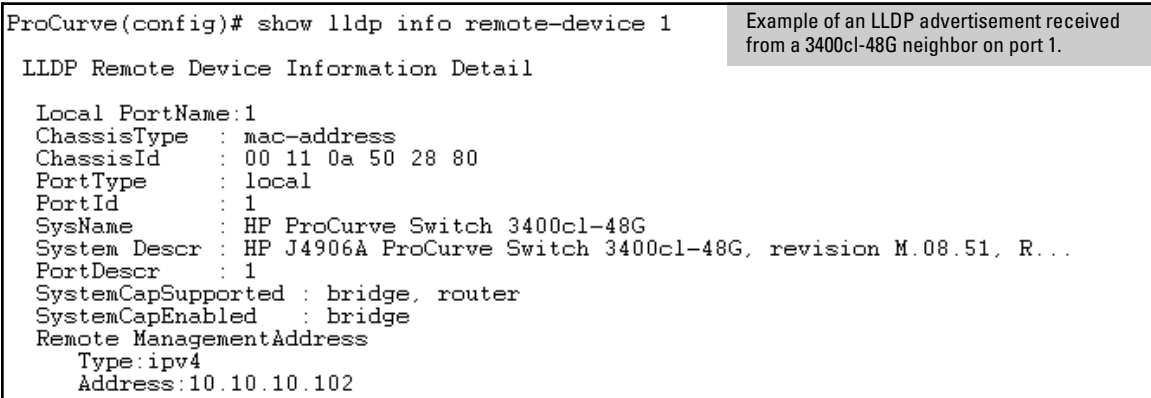
Figure 13-7. Example of a Per-Port Listing of Advertisements Received from an LLDP Device
