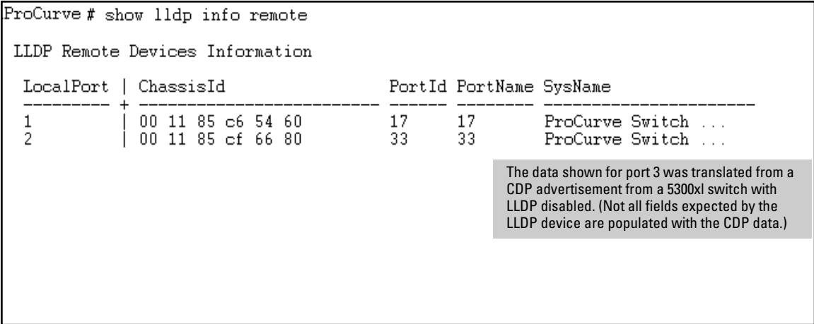
Figure 13-6. Example of a Global Listing of Discovered Devices
