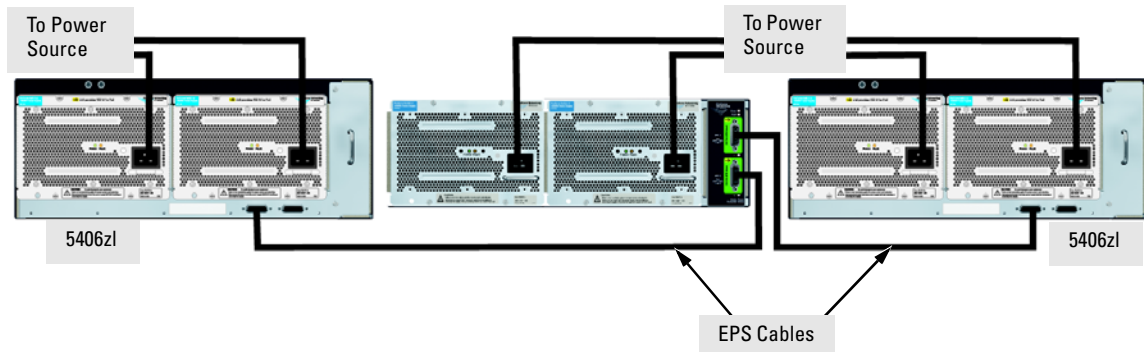
Figure 4-7. Connecting the EPS to two 5406zl switches
