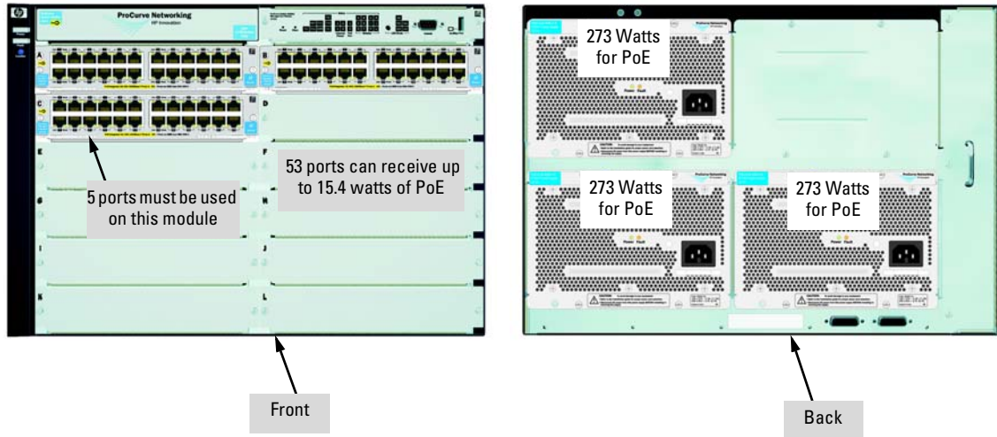
Figure 4-9. Example of a 5412zl with three power supplies, J8712A
