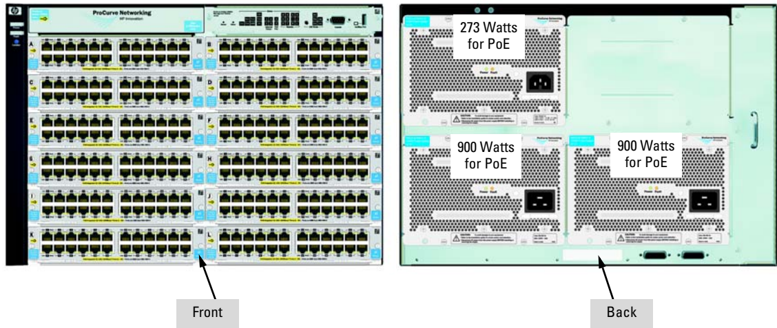
Figure 4-15. Example of a 5412zl with three power supplies (one J8712A and two J8713A)
