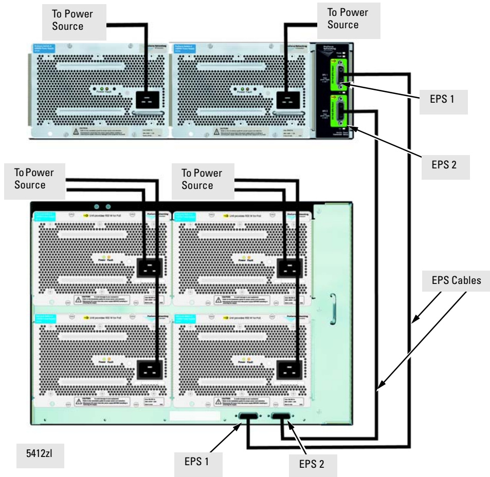
Figure 4-17. Connecting the EPS to one 5412zl switch
