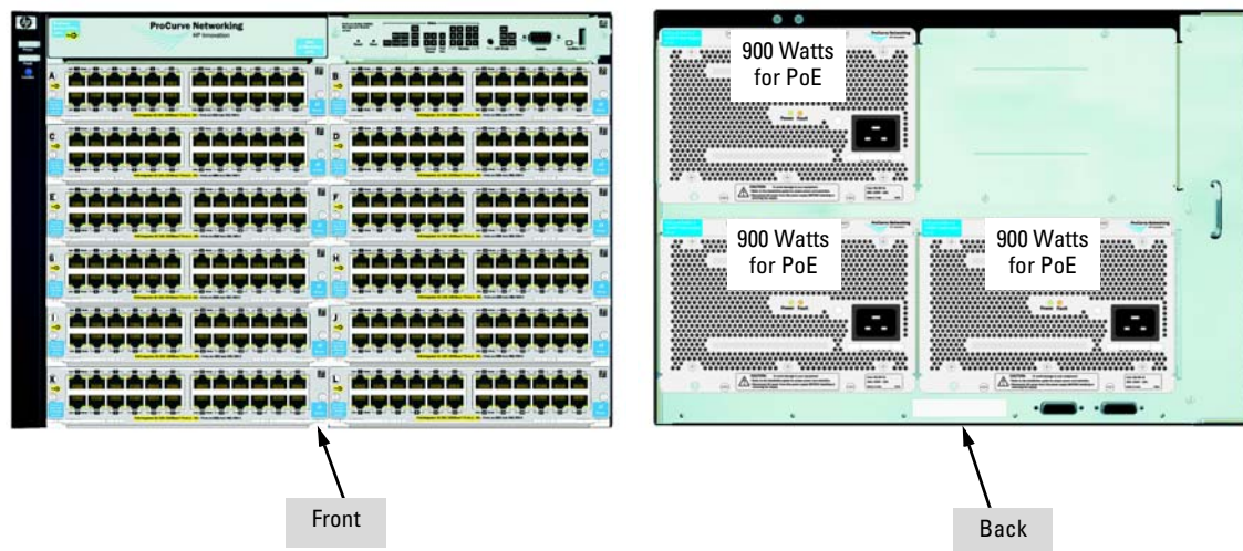
Figure 4-12. Example of a 5412zl with three power supplies, J8713A
