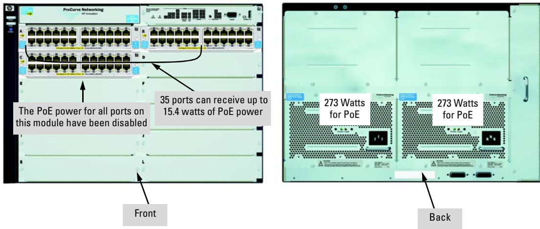
Figure 4-8. Example of a 5412zl with two power supplies, J8712A
