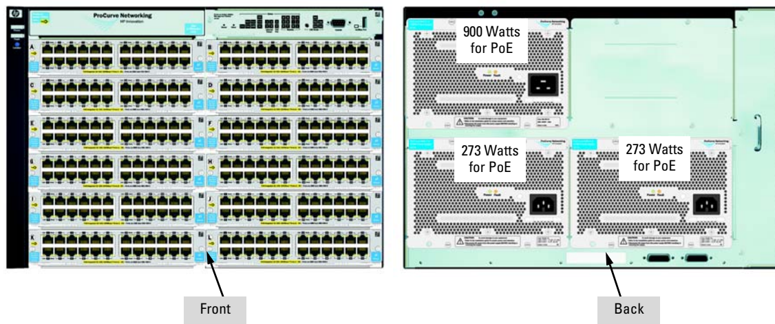
Figure 4-14. Example of a 5412zl with three power supplies (two J8712A and one J8713A)
