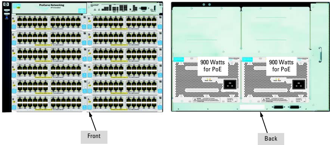
Figure 4-11. Example of a 5412zl with two power supplies, J8713A
