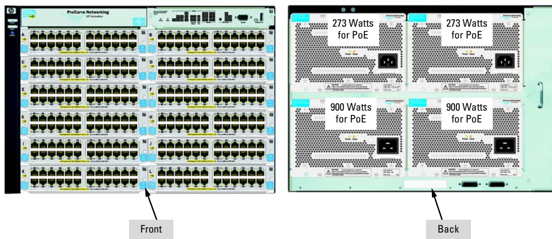
Figure 4-16. Example of a 5412zl with four power supplies (two J8712A and two J8713A)
