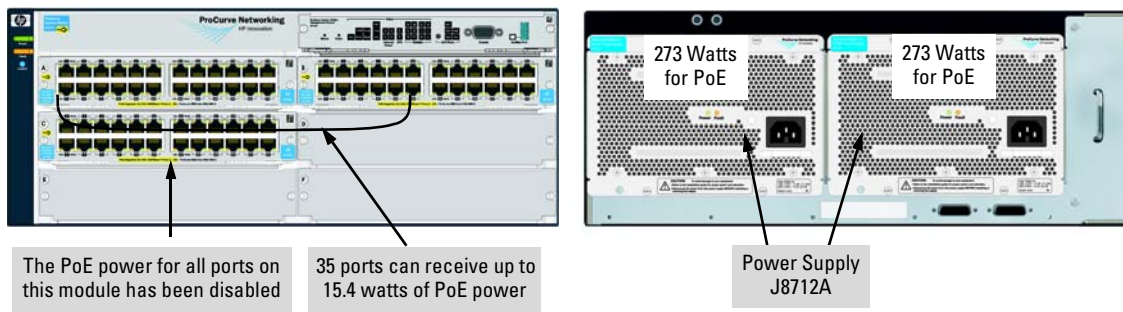
Figure 4-2. Example of a 5406zl with two power supplies, J8712A
