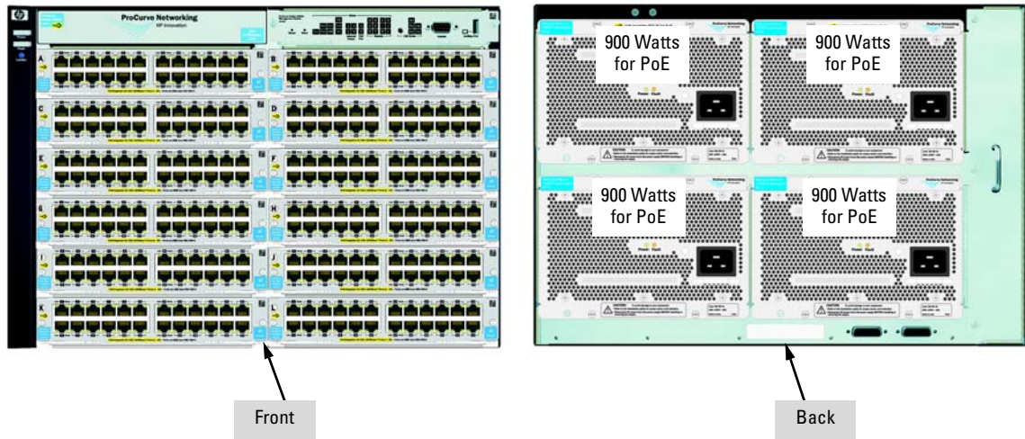
Figure 4-13. Example of a 5412zl with four power supplies, J8713A
