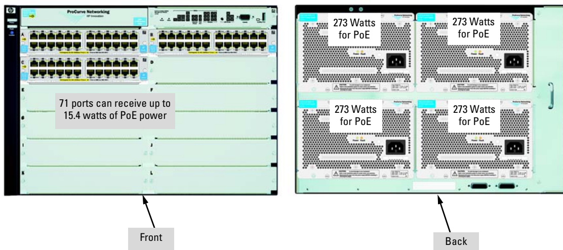
Figure 4-10. Example of a 5412zl with four power supplies, J8712A
