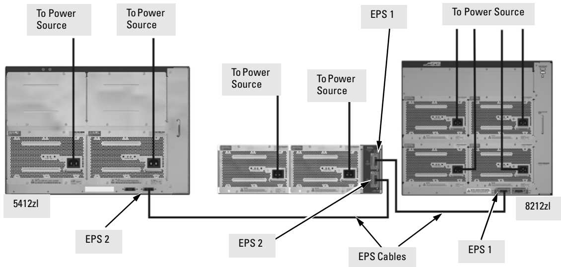
Figure 4-18. Connecting the EPS to two switches, one 5412zl and one 8212zl
