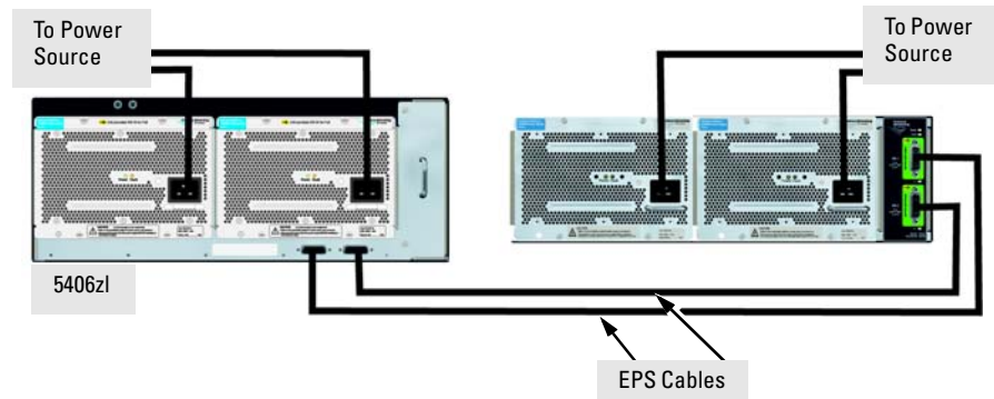
Figure 4-6. Connecting the EPS to one 5406zl switch
