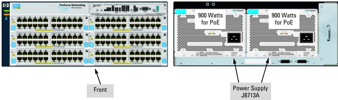
Figure 4-4. Example of a 5406zl with two power supplies, J8713A
