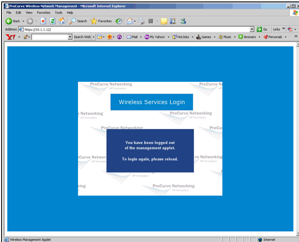
Figure 1. IE Browser
