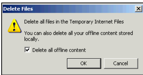
Figure 3. Delete Files
