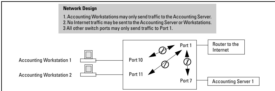
Figure 1. Network Configuration for Named Source-Port Filters Example
