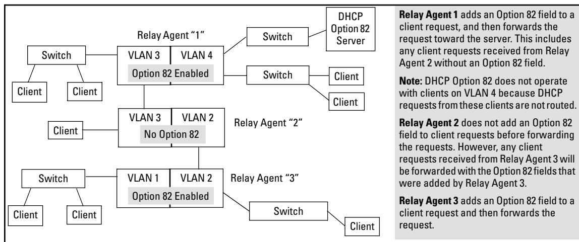
Figure 4. Example of DHCP Option 82 Operation in a Network with a Non-Compliant Relay Agent
