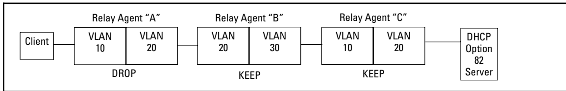
Figure 7. Example Configured To Allow Only the Primary Relay Agent To Contribute an Option 82 Field
