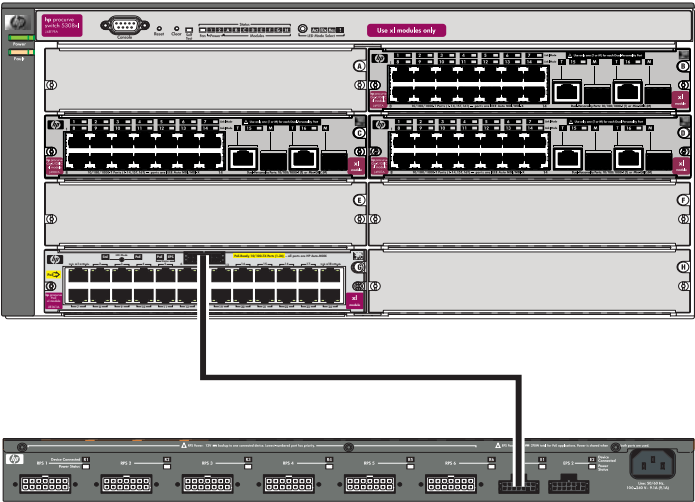
Figure 3-7. Example of an 600 RPS/EPS Powering One Module
