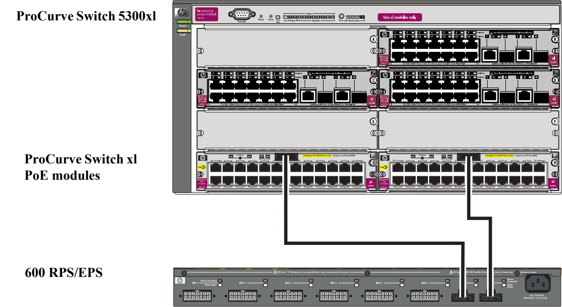
Figure 3-8. Example of an 600 RPS/EPS Powering Two Modules
