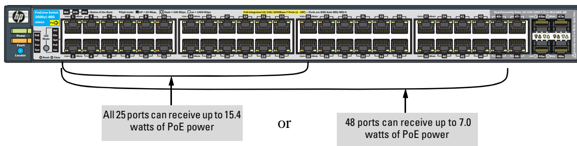
Figure 3-3. Example of a 3500yl-48G-PWR Switch
