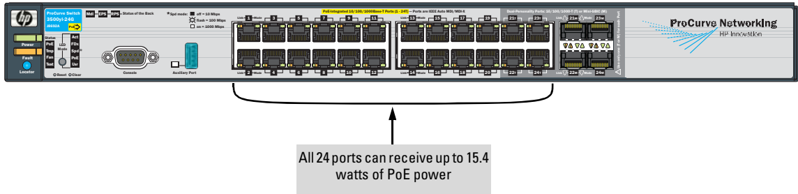
Figure 3-1. Example of a 3500yl-24G-PWR Switch
