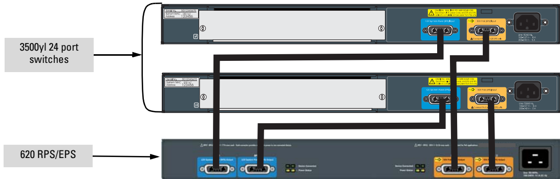
Figure 3-2. Example of two 3500yl-24G-PWR Switches connecting to a ProCurve 620 External and Redundant Power Supply (J8696A)
