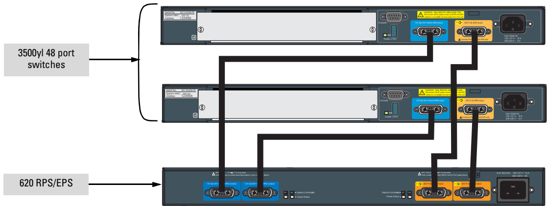
Figure 3-4. Example of two 3500yl-48G-PWR Switches connecting to a ProCurve 620 External and Redundant Power Supply (J8696A)
