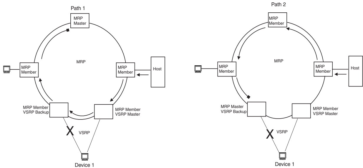
Figure 6 VSRP on MRP rings that failed over
