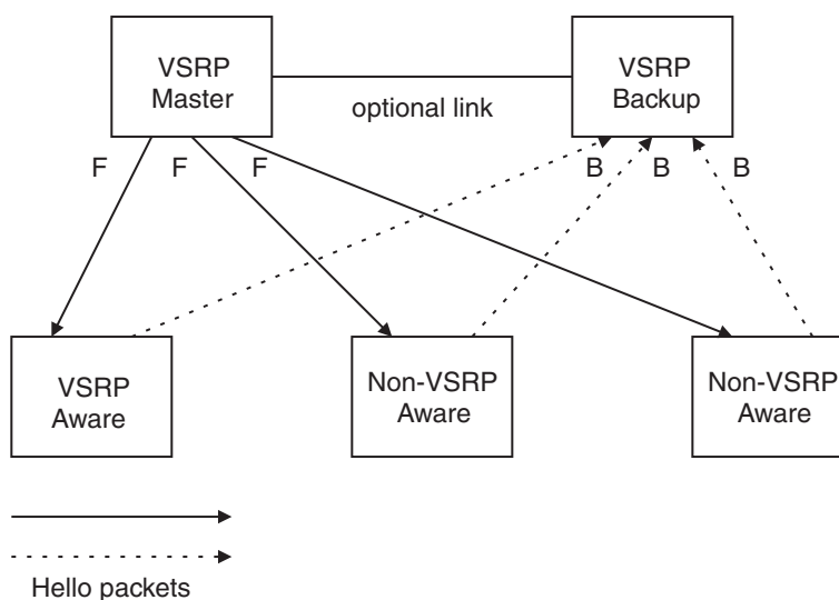
Figure 8 VSRP mesh – redundant paths for Layer 2 and Layer 3 traffic
