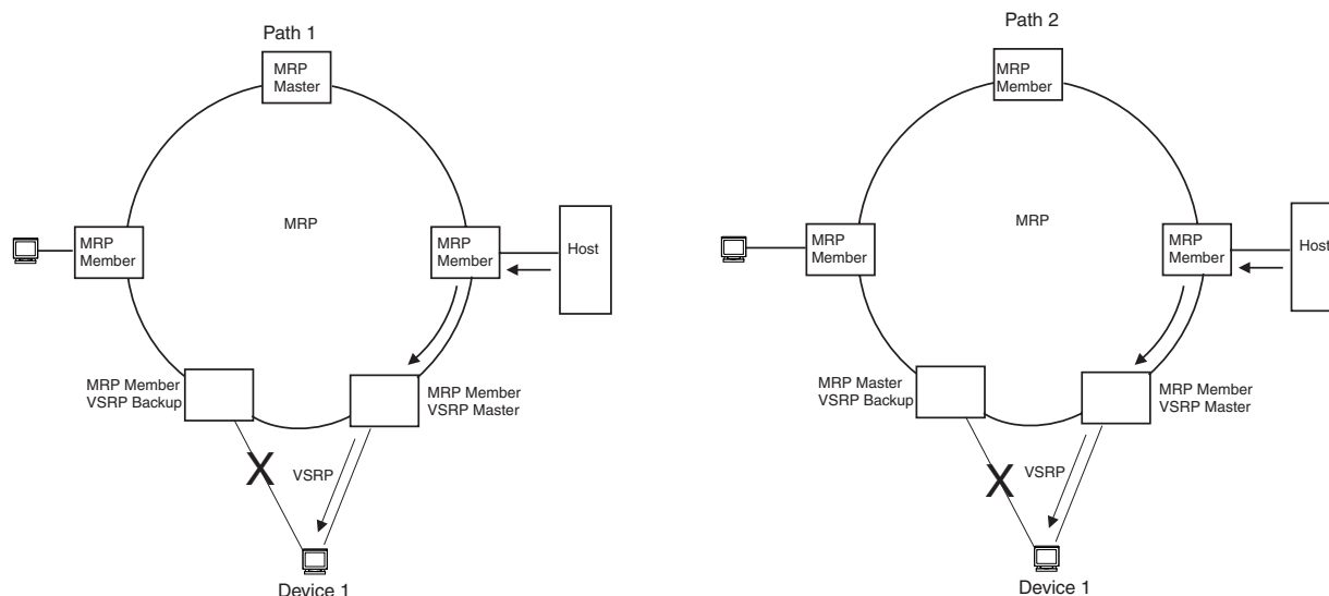
Figure 7 New path established
