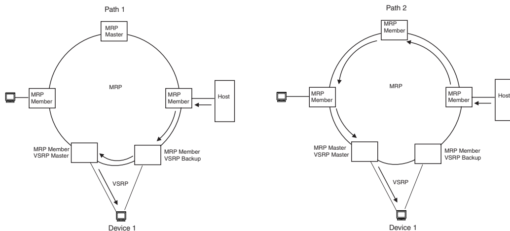
Figure 5 Two data paths from host on an MRP ring to a VSRP-linked device
