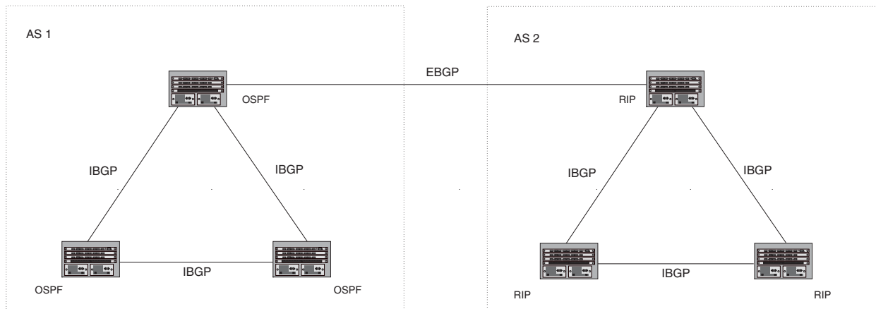
Figure 9.1 Example BGP4 ASs
