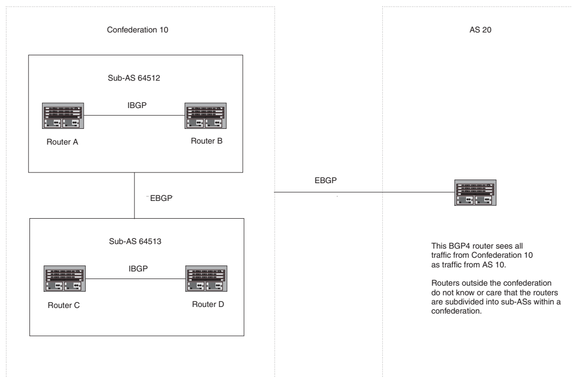
Figure 9.4 Example BGP4 confederation
