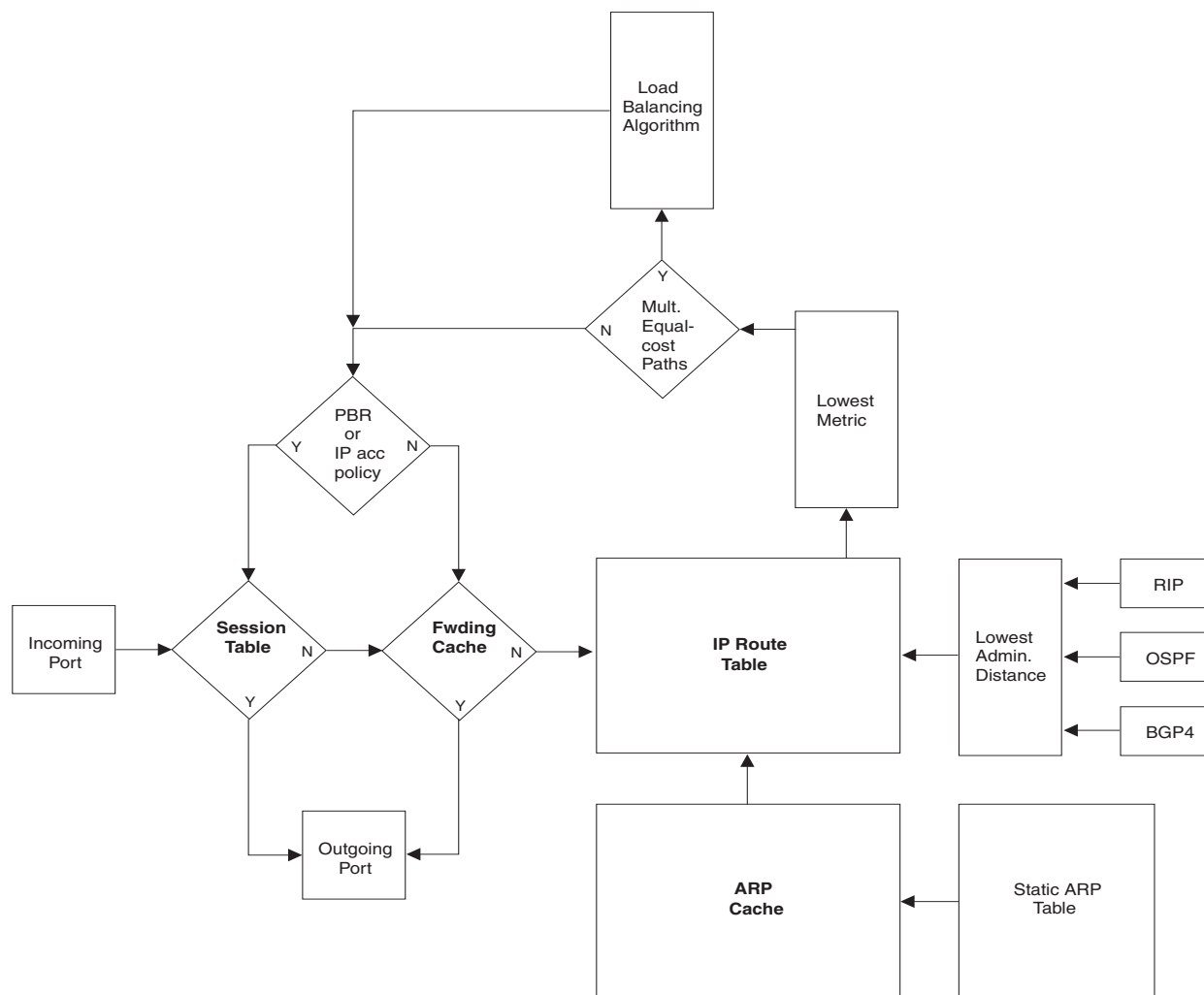
Figure 5.1 IP Packet flow through an HP Routing Switch
