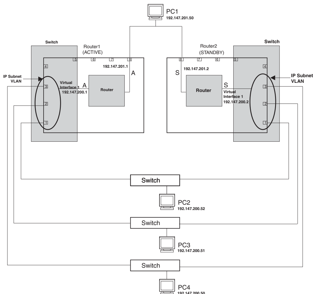
Figure 13.2 Virtual interface providing a redundant link
