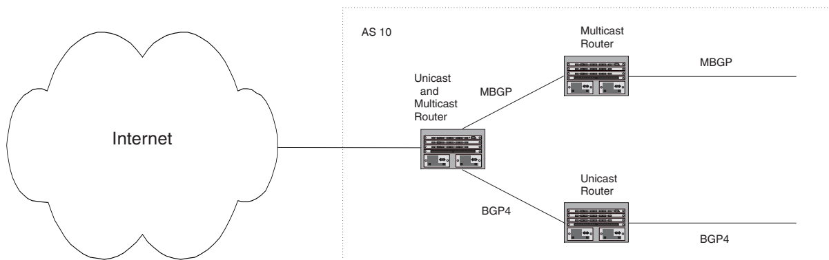
Figure 10.1 MBGP used when multicast topology is different from unicast topology
