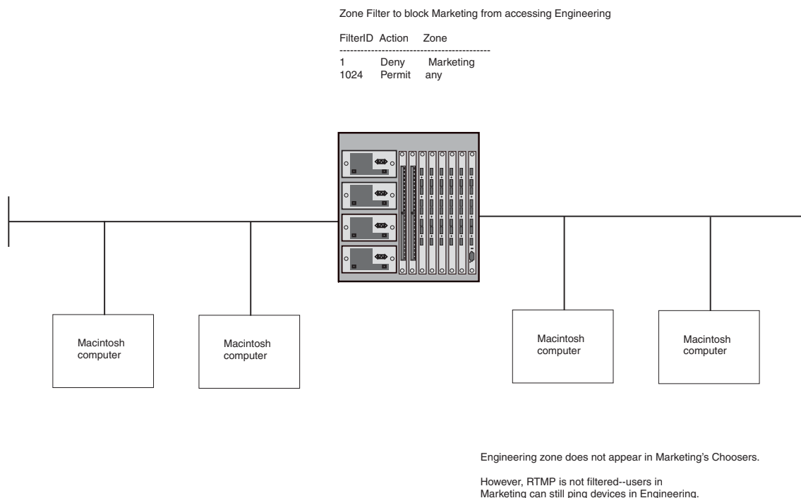
Figure B.8 AppleTalk zone filter
