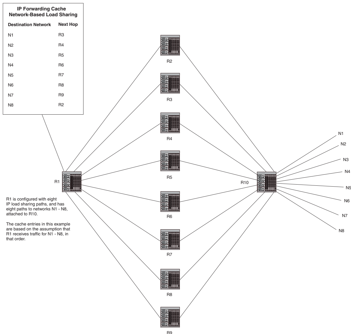
Figure 5.8 Network-based IP load sharing – example with eight equal-cost paths and eight destination networks
