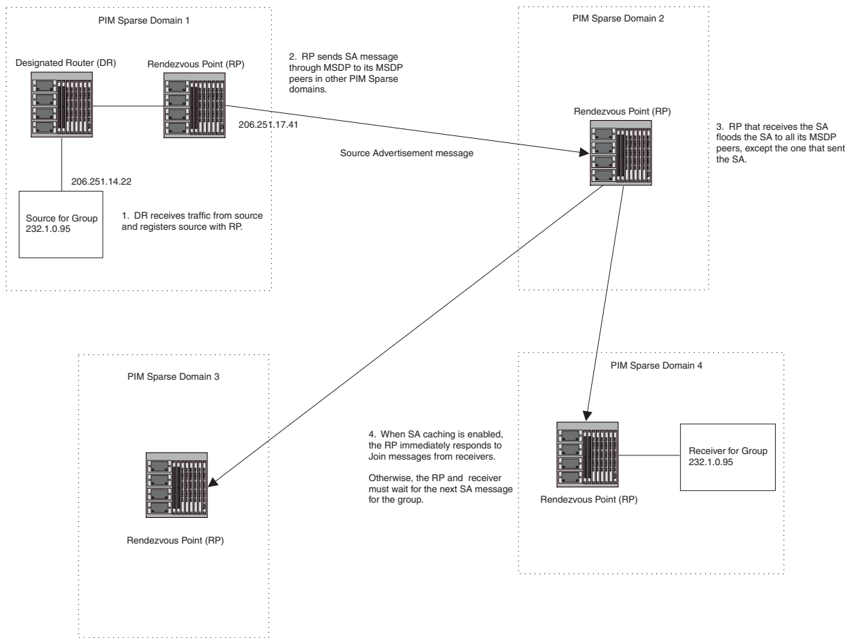
Figure 7.4 PIM Sparse domains joined by MSDP routers
