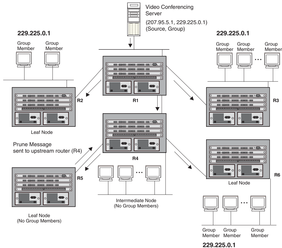
Figure 7.6 Pruning leaf nodes from a multicast tree
