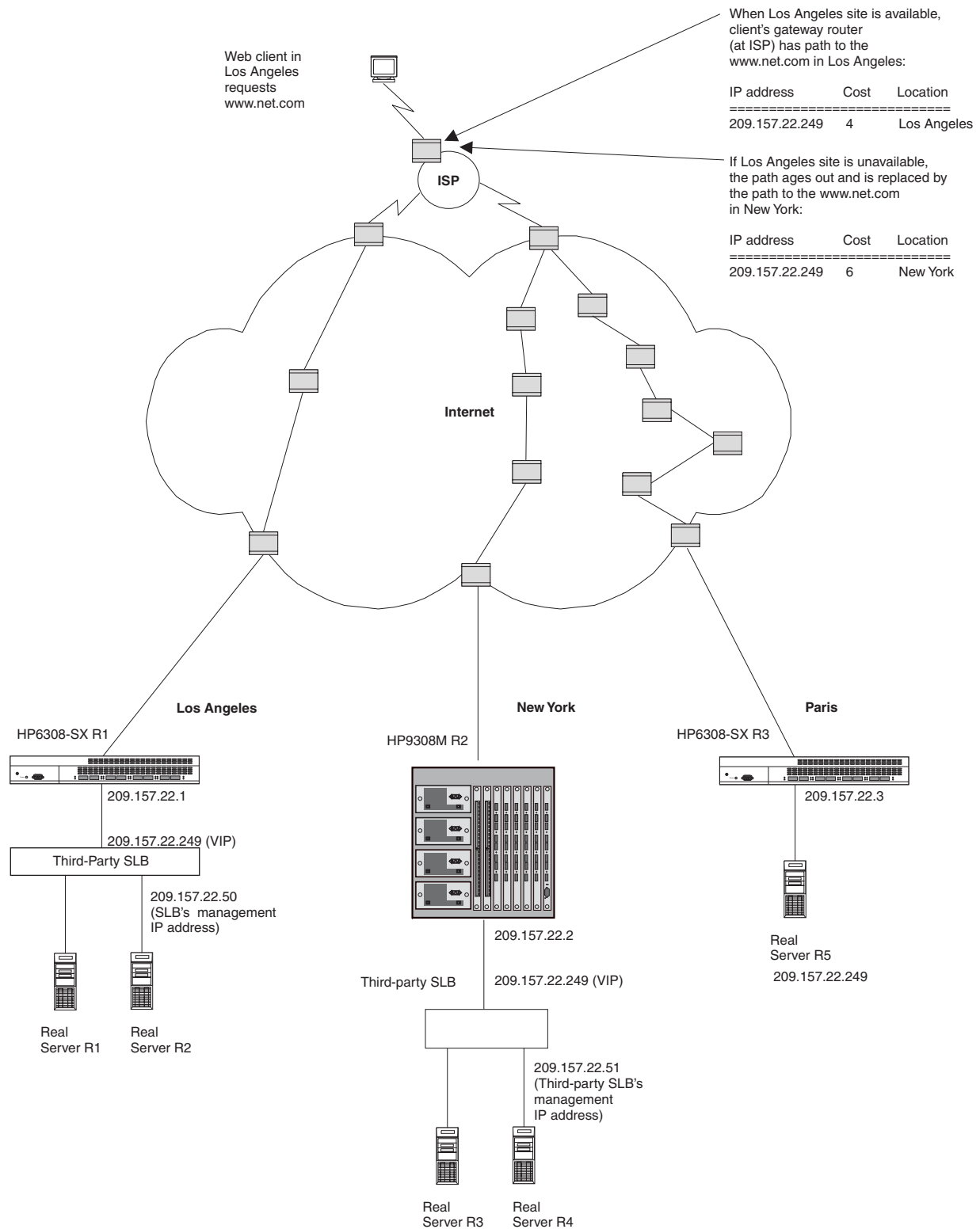
Figure 16.1 Route health injection configuration
