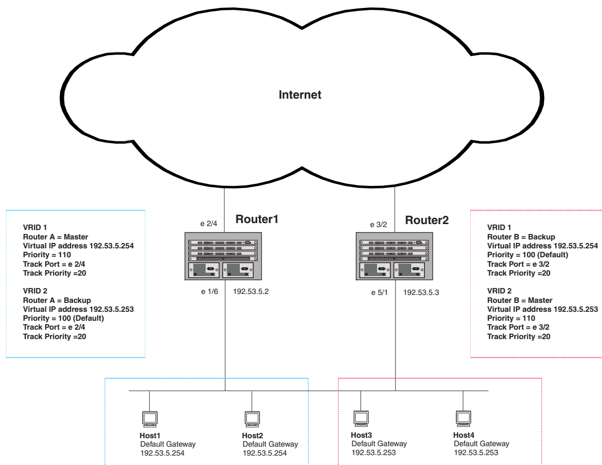
Figure 12.3 Router1 and Router2 are configured to provide dual redundant network access for the host
