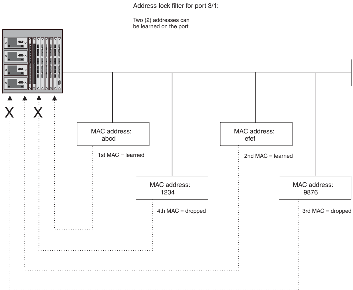
Figure B.5 Address-lock filter
