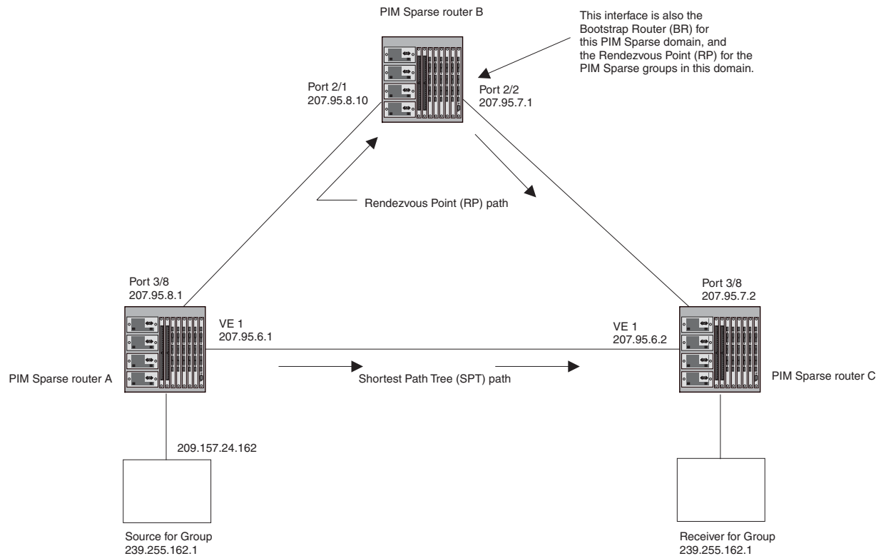
Figure 7.3 Example PIM Sparse domain
