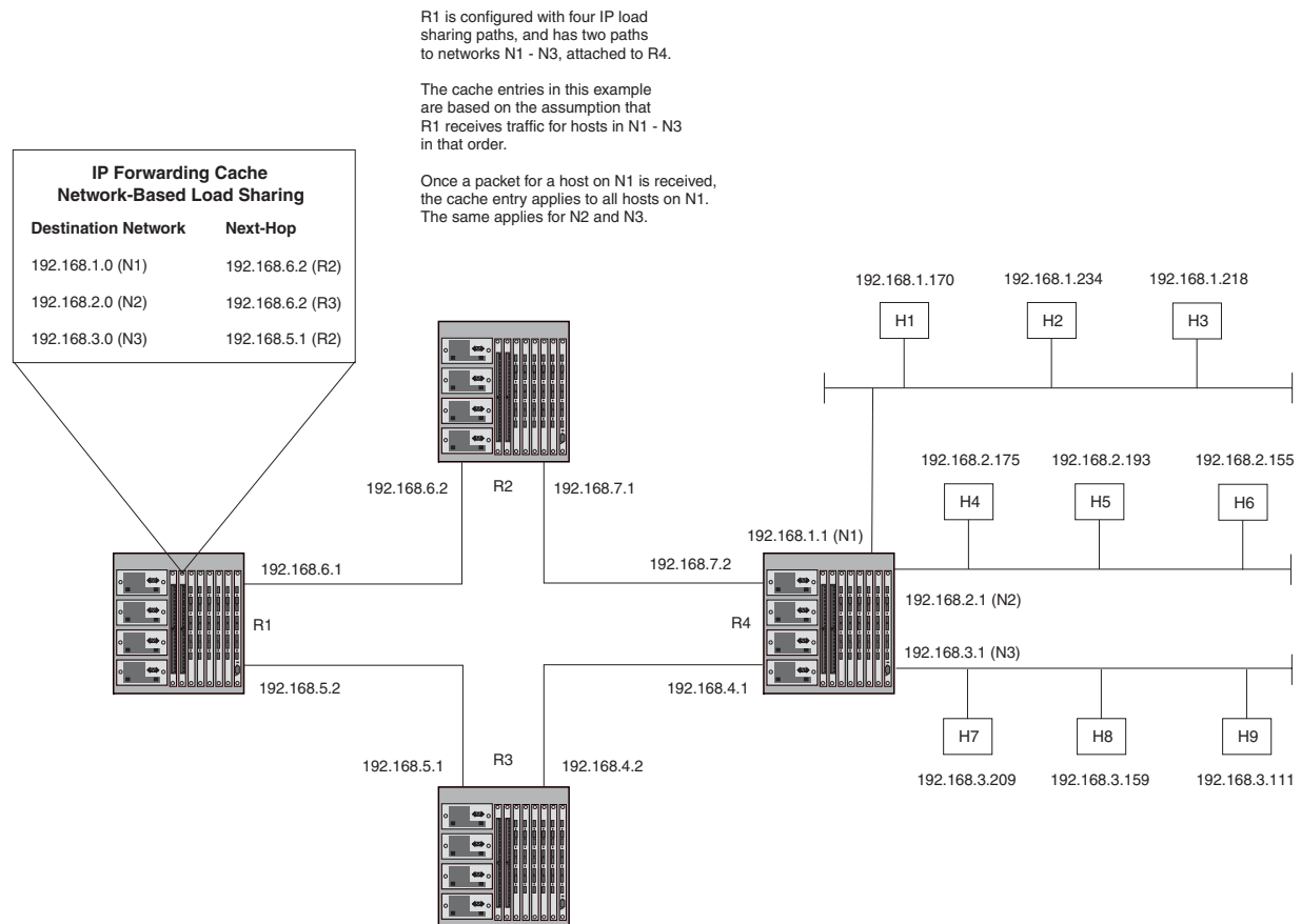
Figure 5.7 Network-based IP load sharing – basic example
