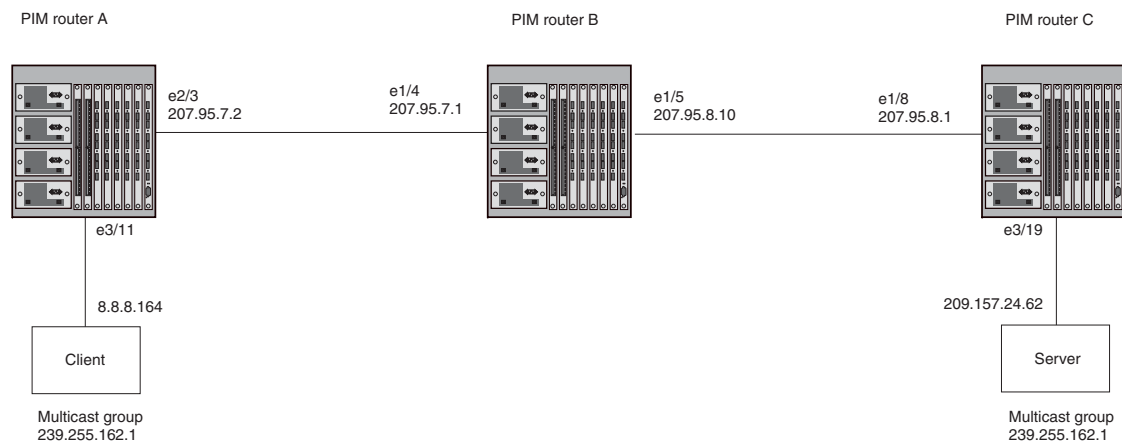
Figure 7.9 Example PIM Group
