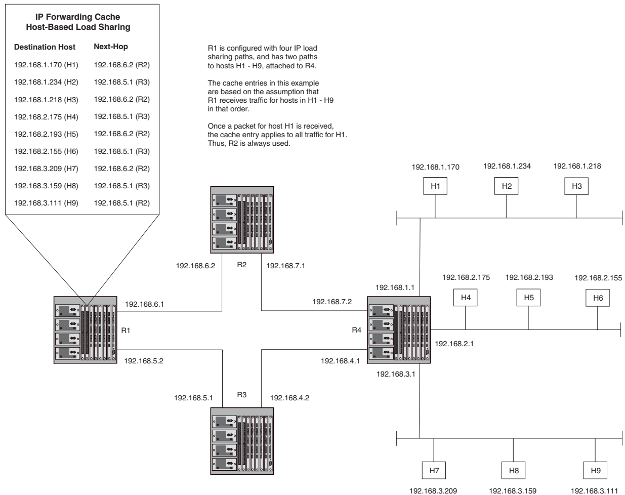
Figure 5.5 Host-based IP load sharing – basic example
