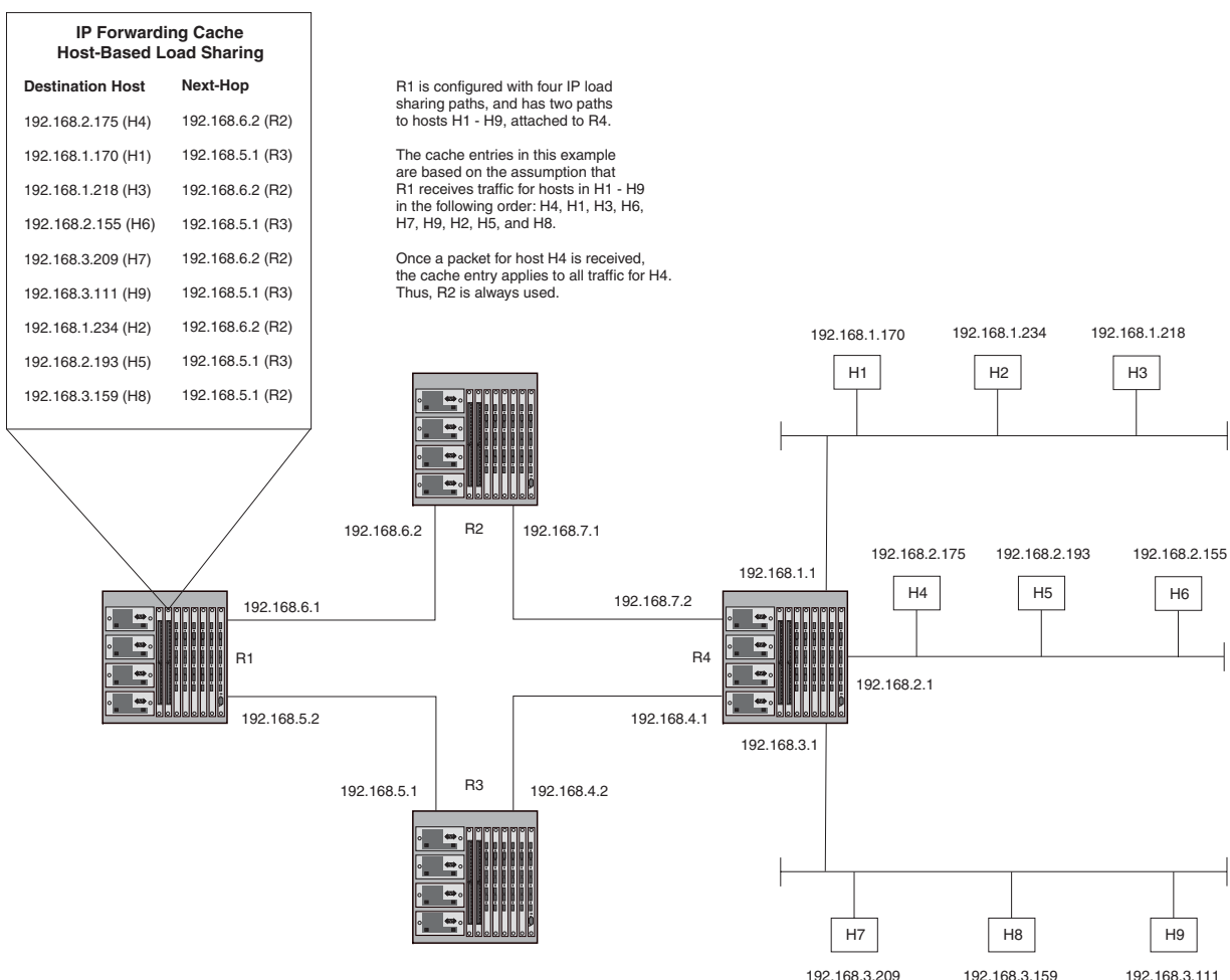
Figure 5.6 Host-based IP load sharing – additional example
