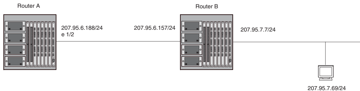
Figure 5.2 Example of a static route
