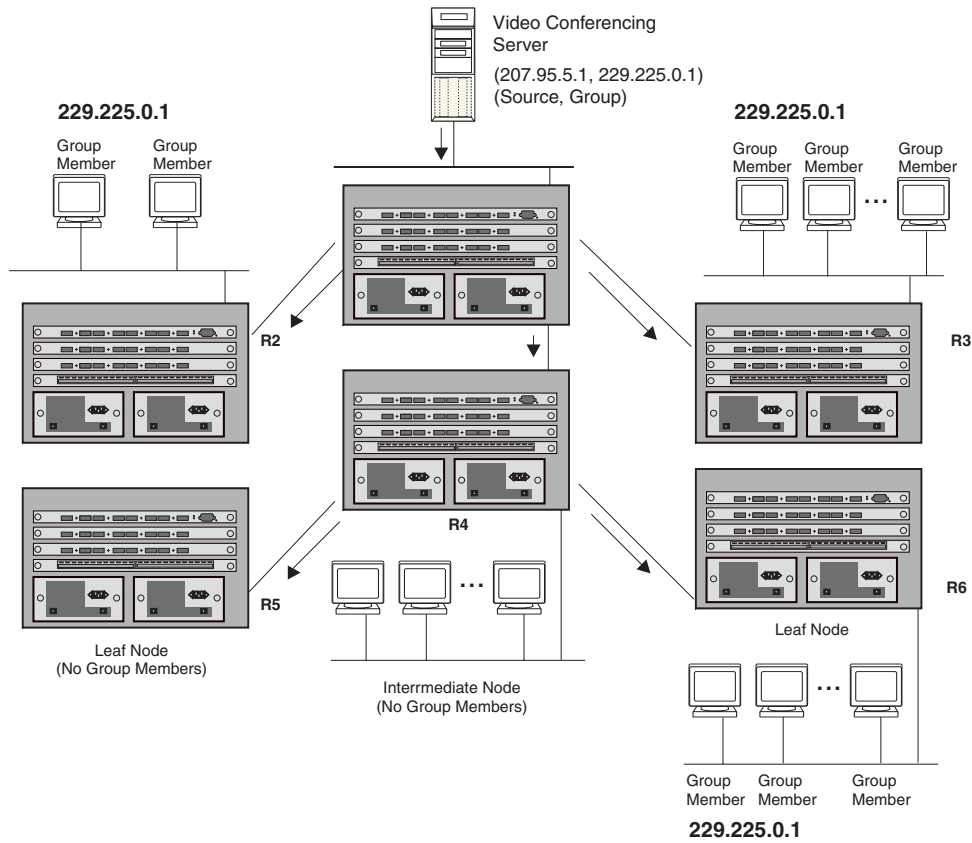
Figure 7.5 Downstream broadcast of IP multicast packets from source host
