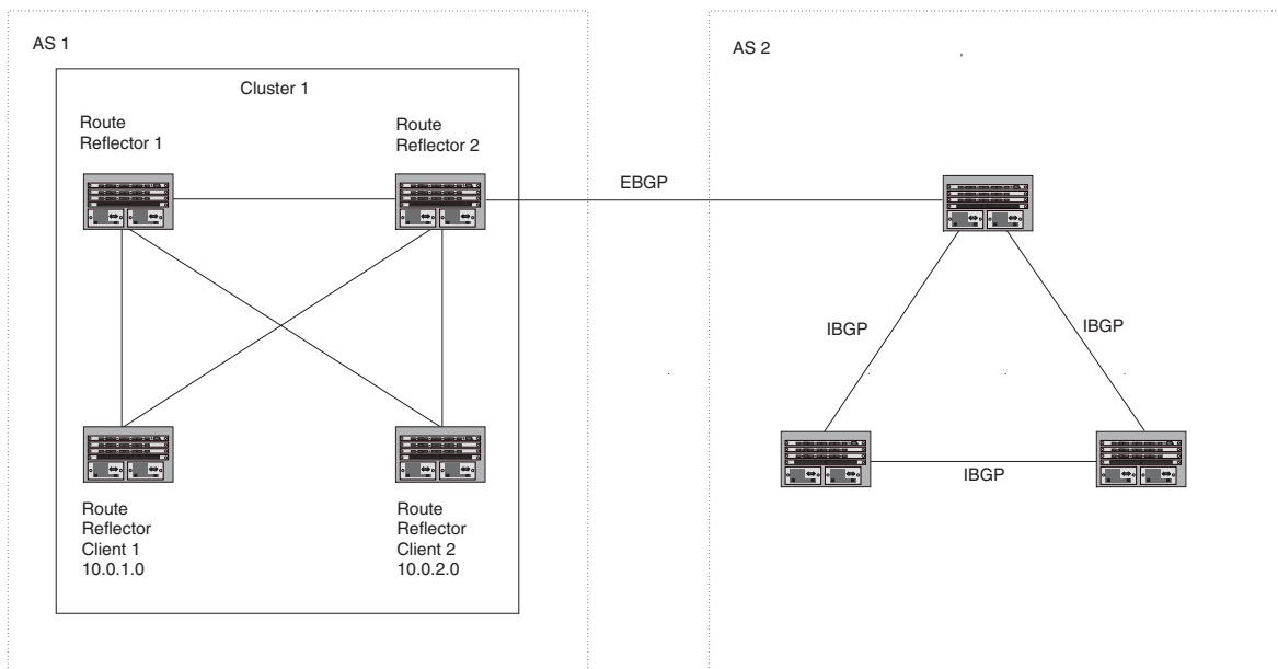
Figure 9.3 Example route reflector configuration
