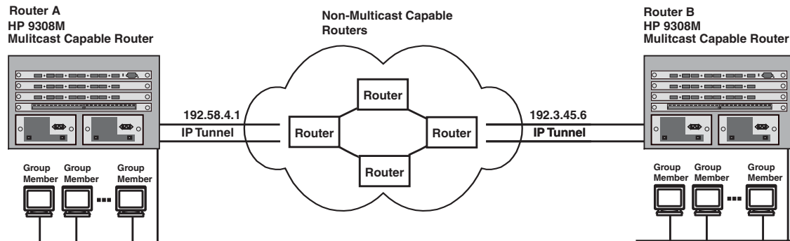
Figure 7.7 IP in IP tunneling on multicast packets in a unicast network
