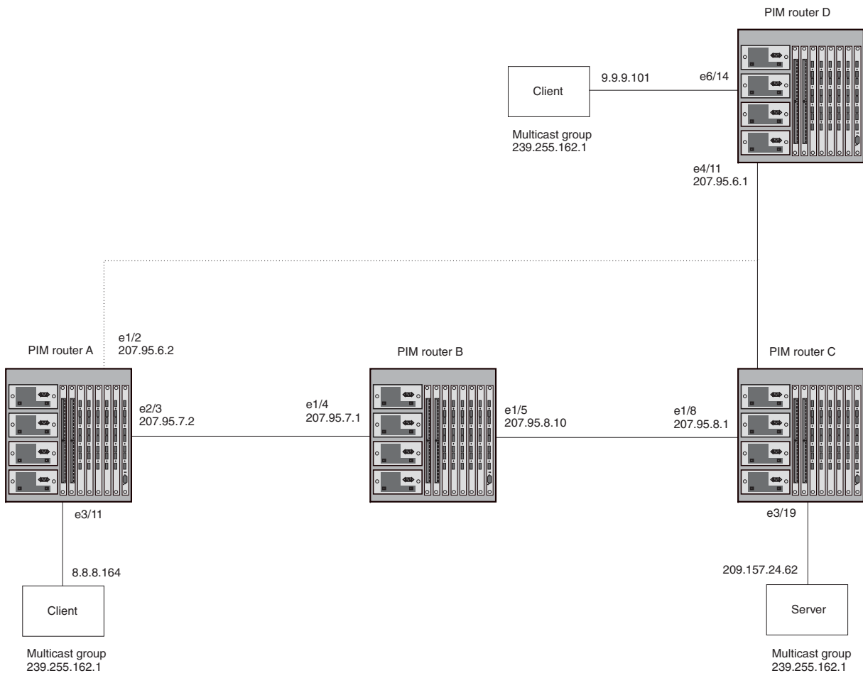
Figure 7.8 Example multicast static routes
