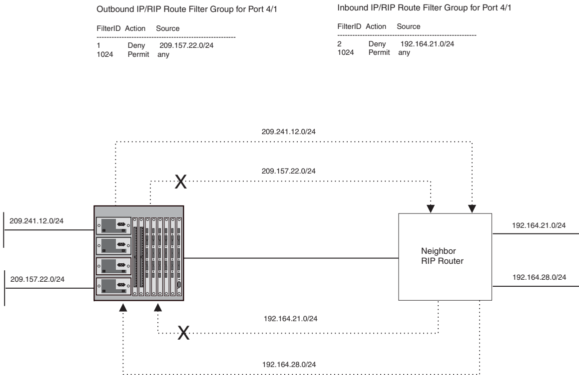
Figure B.6 RIP route filters
