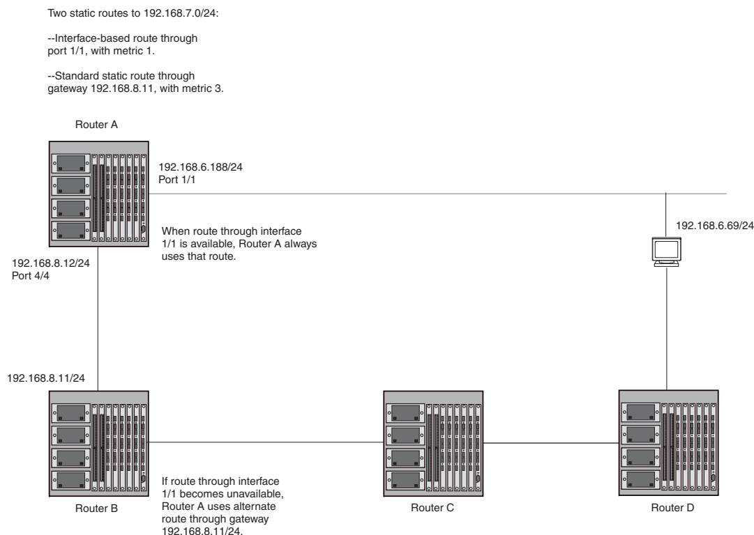
Figure 5.4 Standard and interface routes to the same destination network
