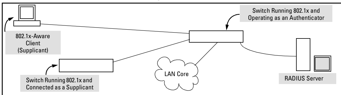
Figure 5-1. Example of an 802.1x Application
