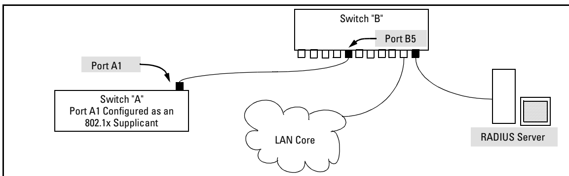
Figure 5-4. Example of Supplicant Operation
