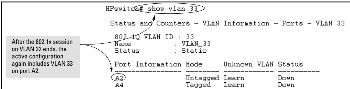
Figure 5-8. The Active Configuration for VLAN 33 Restores Port A2 After the 802.1x Session Ends
