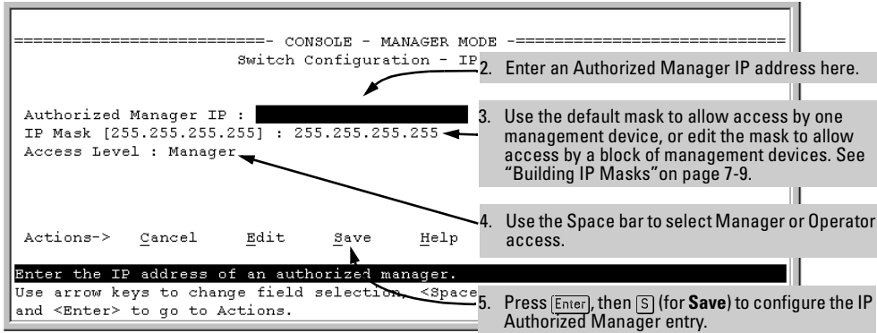
Figure 7-2. Example of How To Add an Authorized Manager Entry (Continued)
