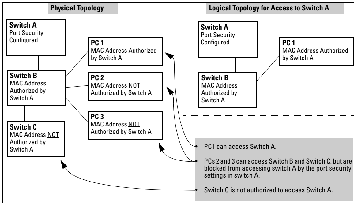
Figure 0-1. Example of How Port Security Controls Access
