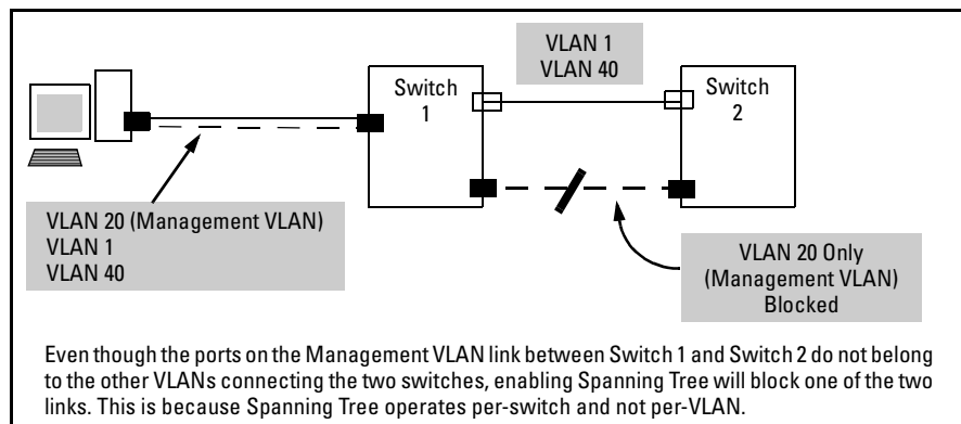
Figure 11-23. Example of Inadvertently Blocking a Management VLAN Link by Implementing Spanning Tree
