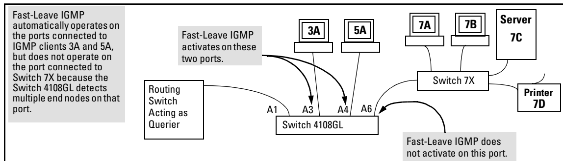
Figure 12-3. Example of Automatic Fast-Leave IGMP Criteria
