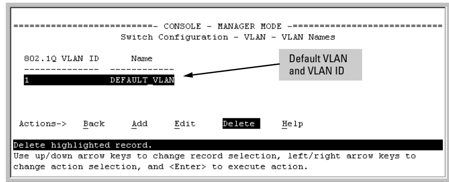
Figure 9-46. The Default VLAN Names Screen
