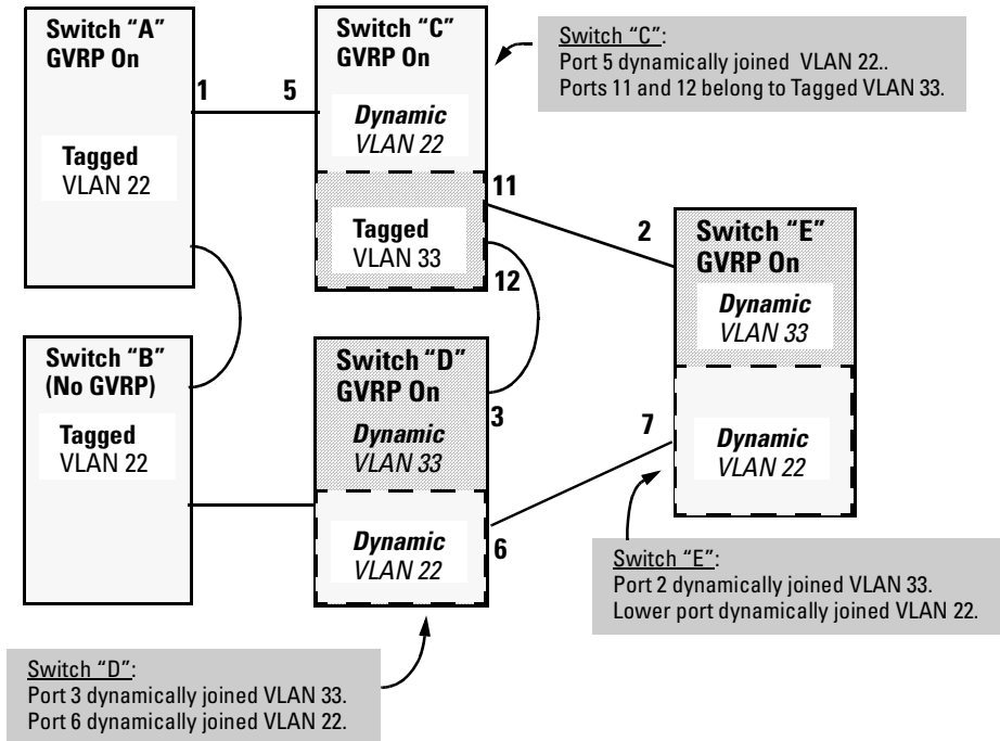
Figure 9-58. Example of GVRP Operation
