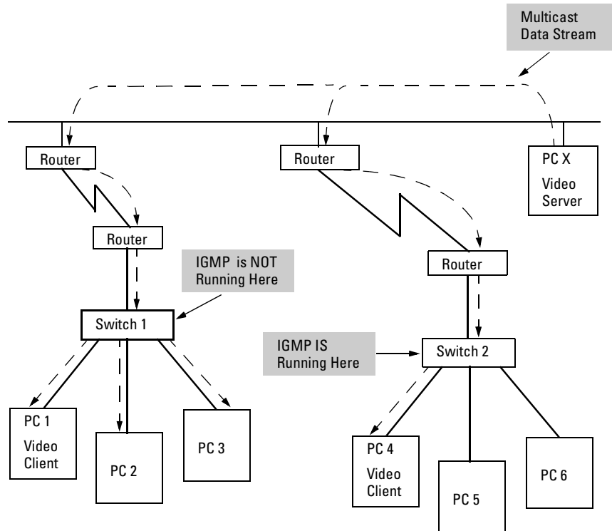
Figure 9-67. The Advantage of Using IGMP
