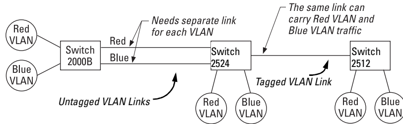
Figure 9-42. Example of Tagged and Untagged VLAN Technology in the Same Network
