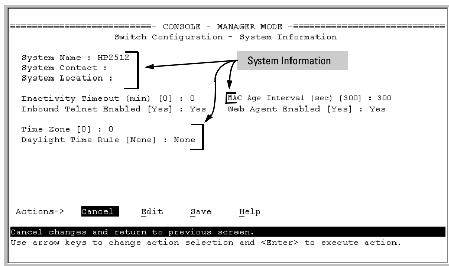
Figure 5-8. The System Information Configuration Screen (Default Values)
