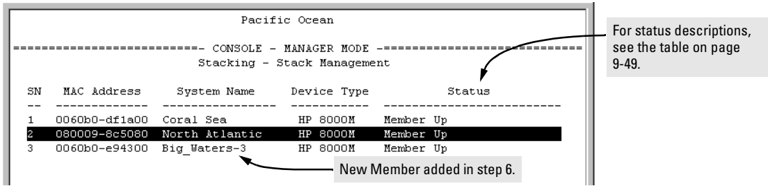
Figure 9-11. Example of Stack Management Screen After New Member Added
