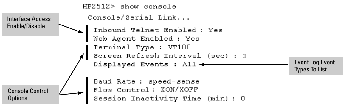
Figure 5-5. Listing of Show Console Command
