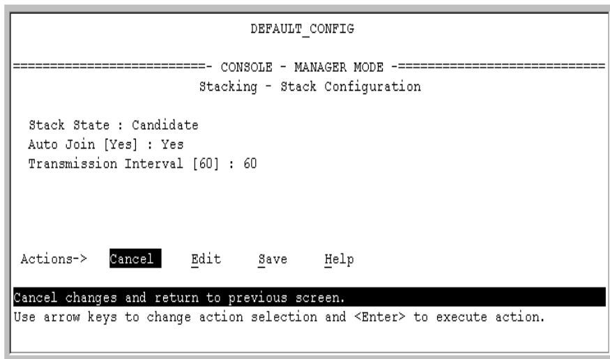
Figure 9-6. The Default Stack Configuration Screen
