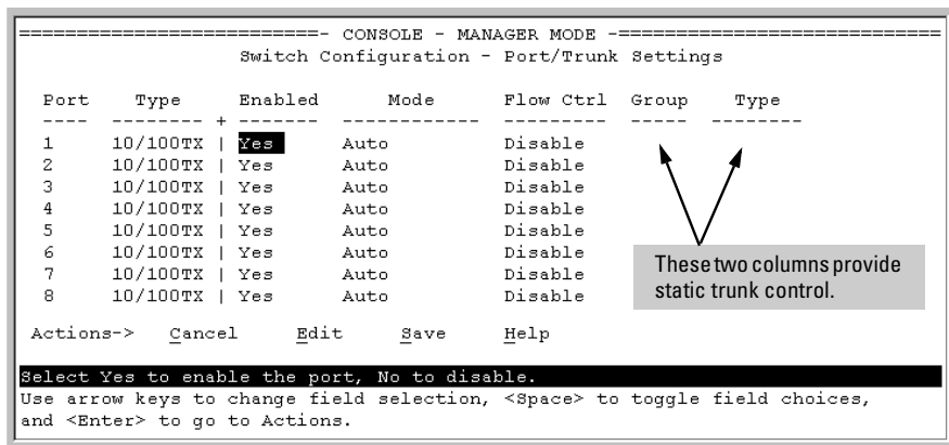
Figure 6-4. Example of the Menu Screen for Configuring a Port Trunk Group
