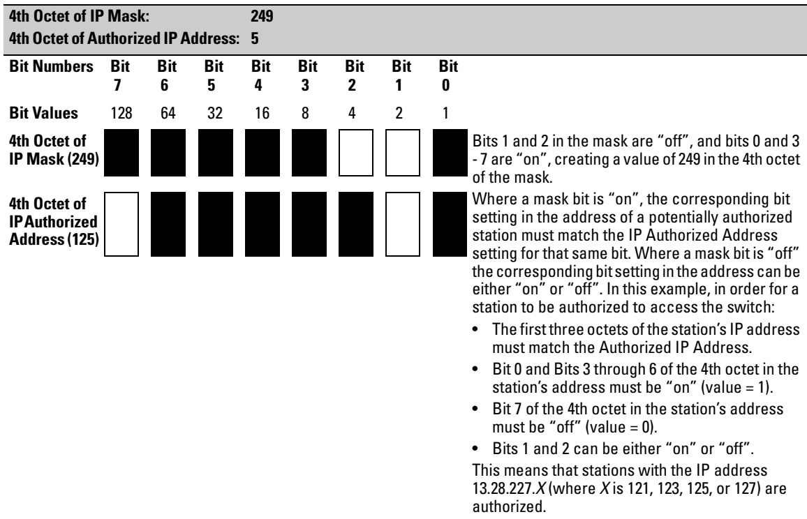
Figure 7-16. Example of How the Bitmap in the IP Mask Defines Authorized Manager Addresses
