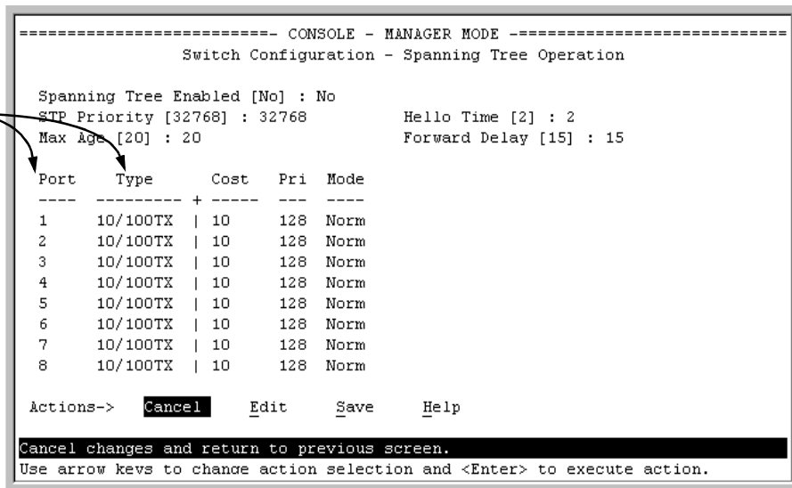
Figure 9-69. Example of the STP Configuration Screen
