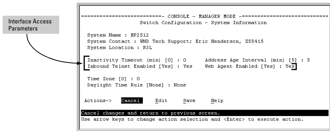
Figure 5-4. The Default Interface Access Parameters Available in the Menu Interface
