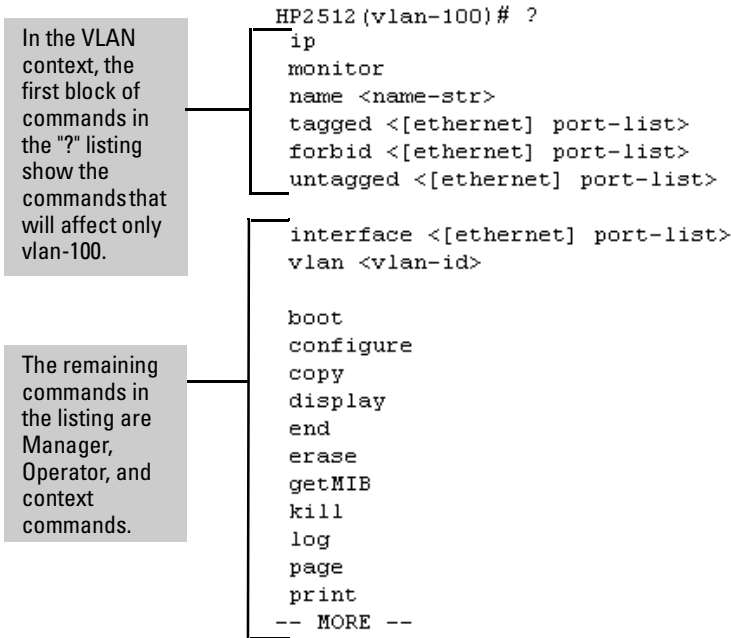
Figure 3-11. Context-Specific Commands Affecting VLAN Context
