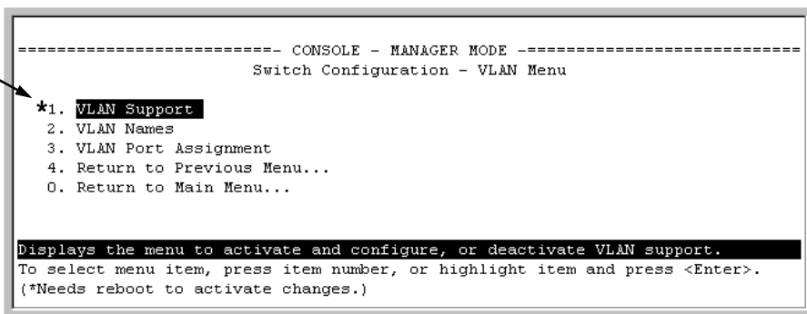
Figure 9-45. VLAN Menu Screen Indicating the Need To Reboot the Switch
