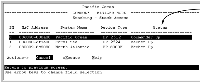
Figure 9-16. Example of the Stack Access Screen
