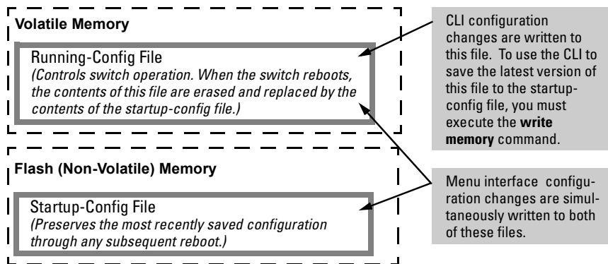
Figure C-10. Conceptual Illustration of Switch Memory Operation
