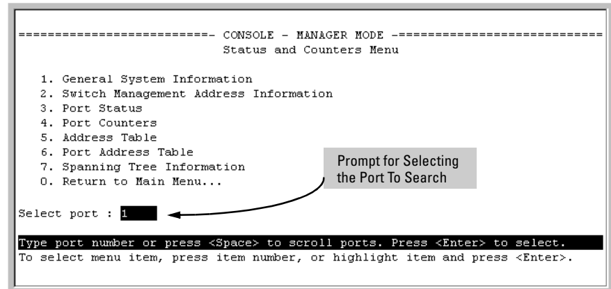
Figure 10-9. Listing MAC Addresses for a Specific Port
