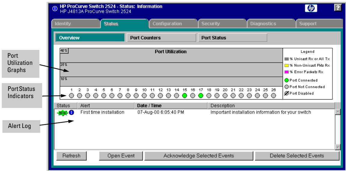
Figure 10-15. Example of a Web Browser Interface Status Overview Screen
