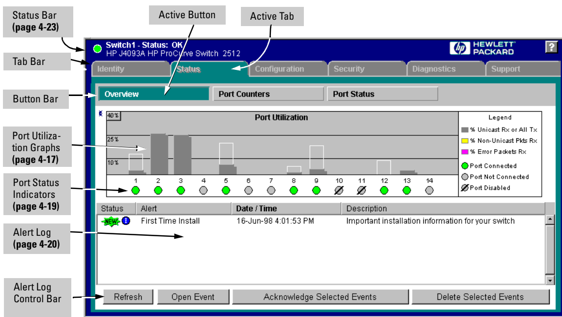
Figure 4-8. The Overview Window
