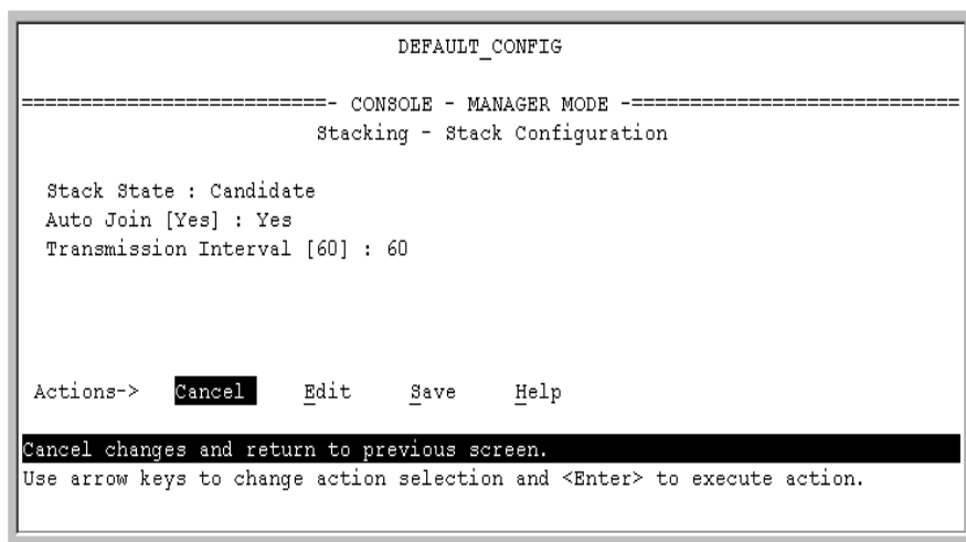
Figure 9-8. The Default Stack Configuration Screen
