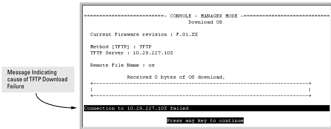
Figure A-18. Example of Message for Download Failure
