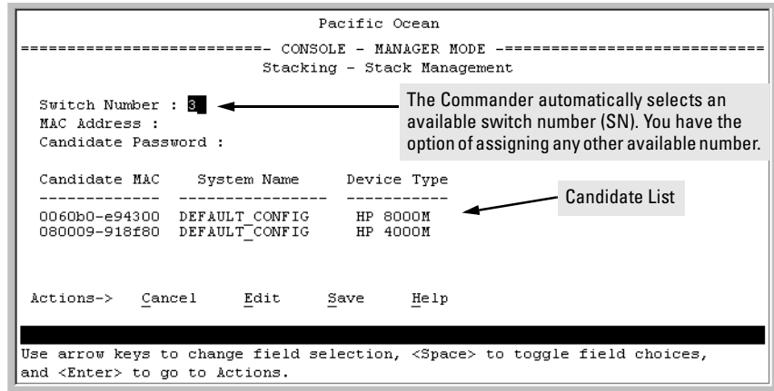
Figure 9-10. Example of Candidate List in Stack Management Screen
