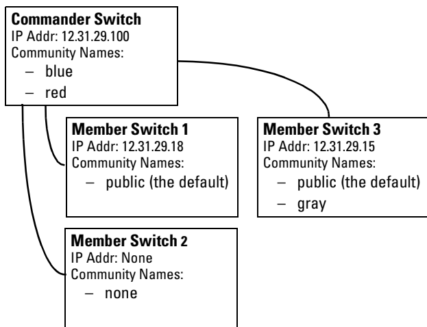
Figure 9-37. Example of SNMP Community Operation with Stacking
