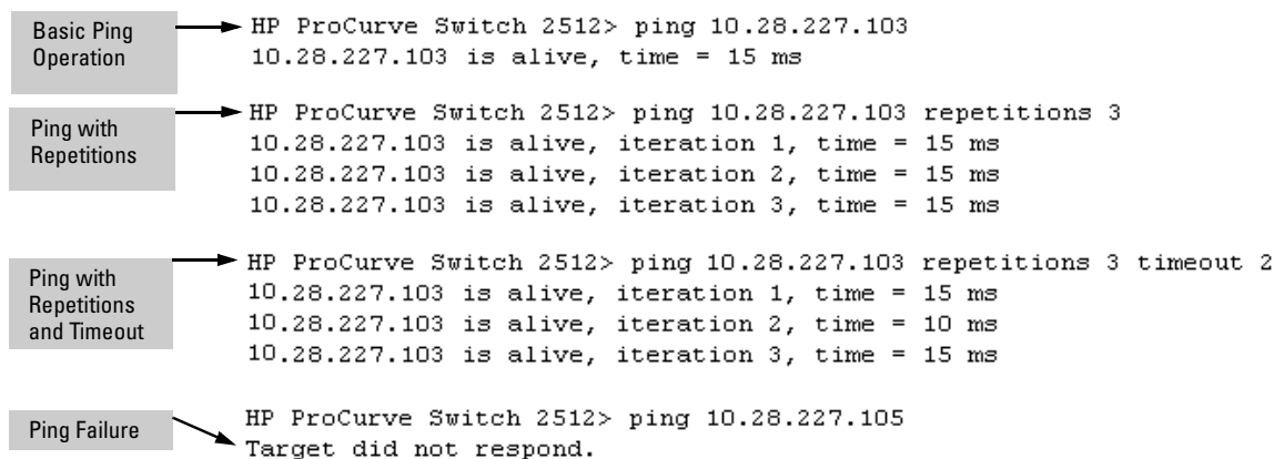
Figure 11-13.Examples of Ping Tests
