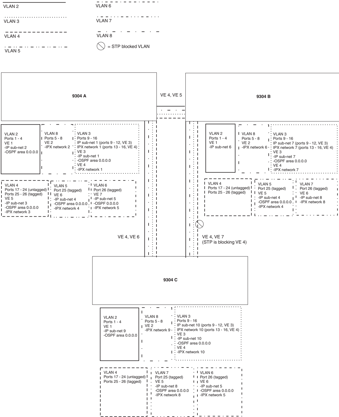
Figure 13.12 Routing between protocol-based VLANs
