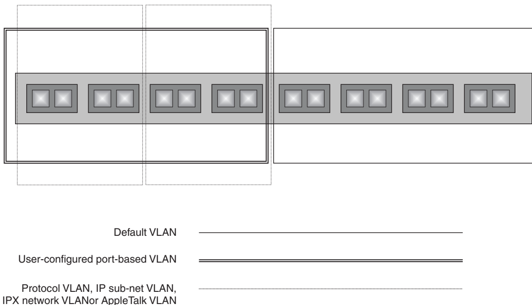
Figure 13.2 Layer 3 protocol VLANs within a Layer 2 port-based VLAN
