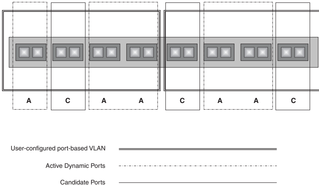
Figure 13.8 Protocol VLAN with “leaky” (dynamic) ports
