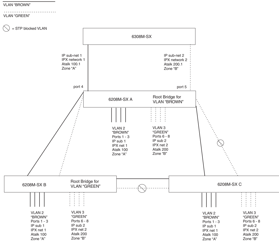
Figure 13.10 More complex port-based VLAN
