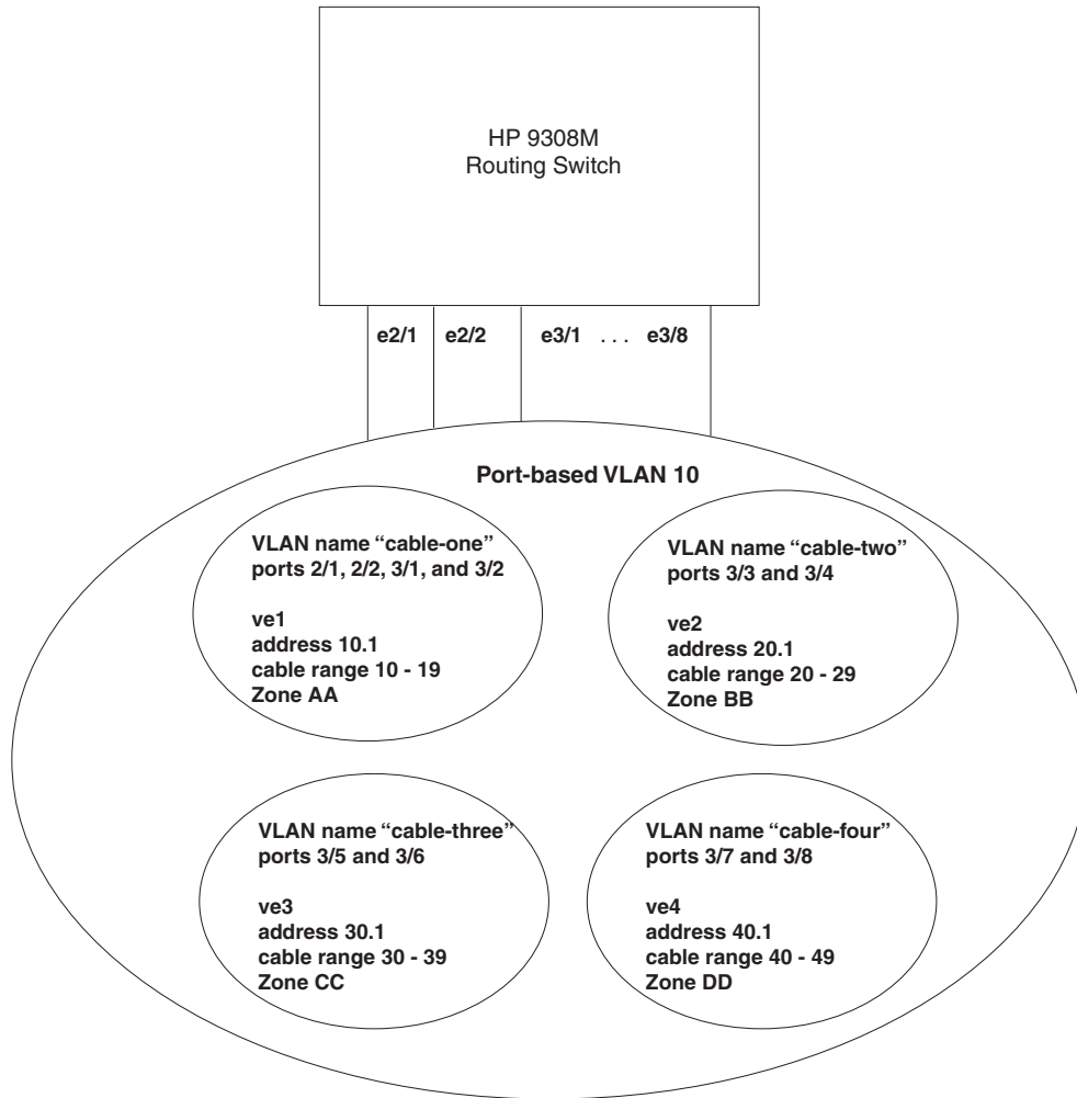
Figure 13.13 AppleTalk Cable VLANs
