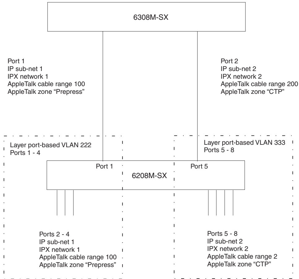
Figure 13.9 Port-based VLANs 222 and 333
