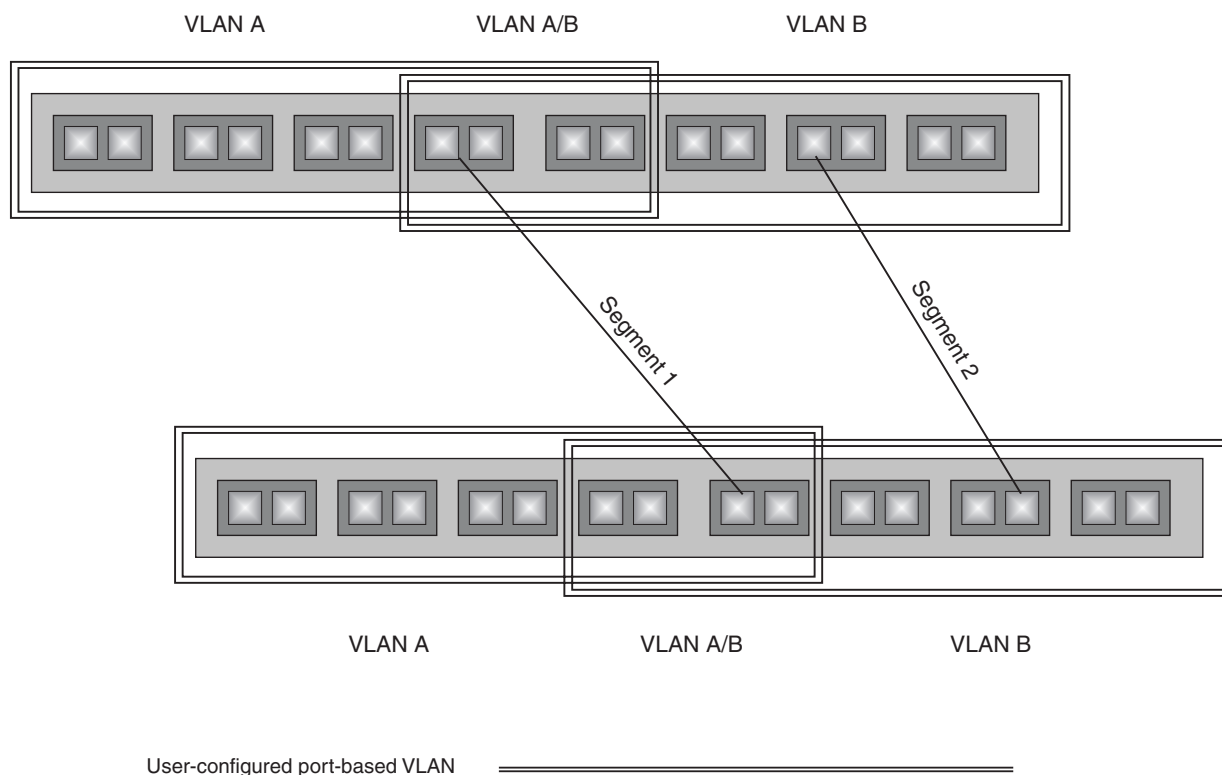
Figure 13.5 VLANs configured across multiple devices
