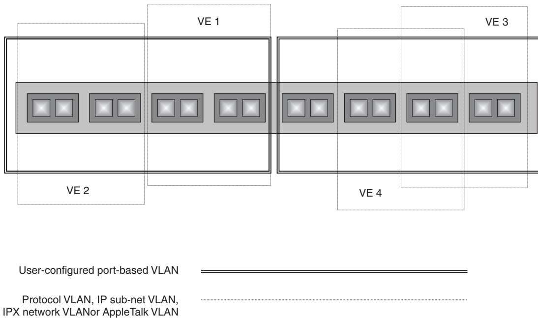
Figure 13.6 Use virtual interfaces for routing between Layer 3 protocol VLANs
