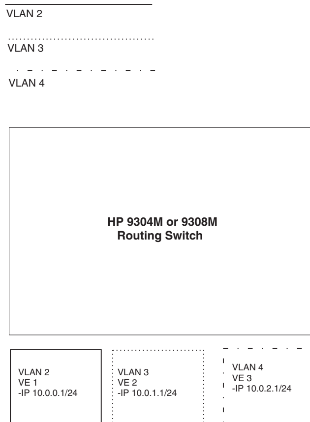
Figure 13.14 Multiple port-based VLANs with separate protocol addresses
