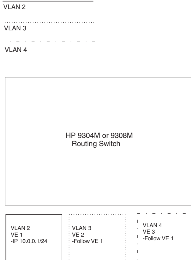
Figure 13.15 Multiple port-based VLANs with the same protocol address
