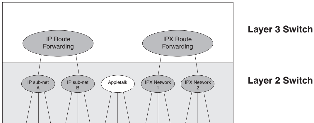
Figure 6.3 Logical representation of ISR within routing switches
