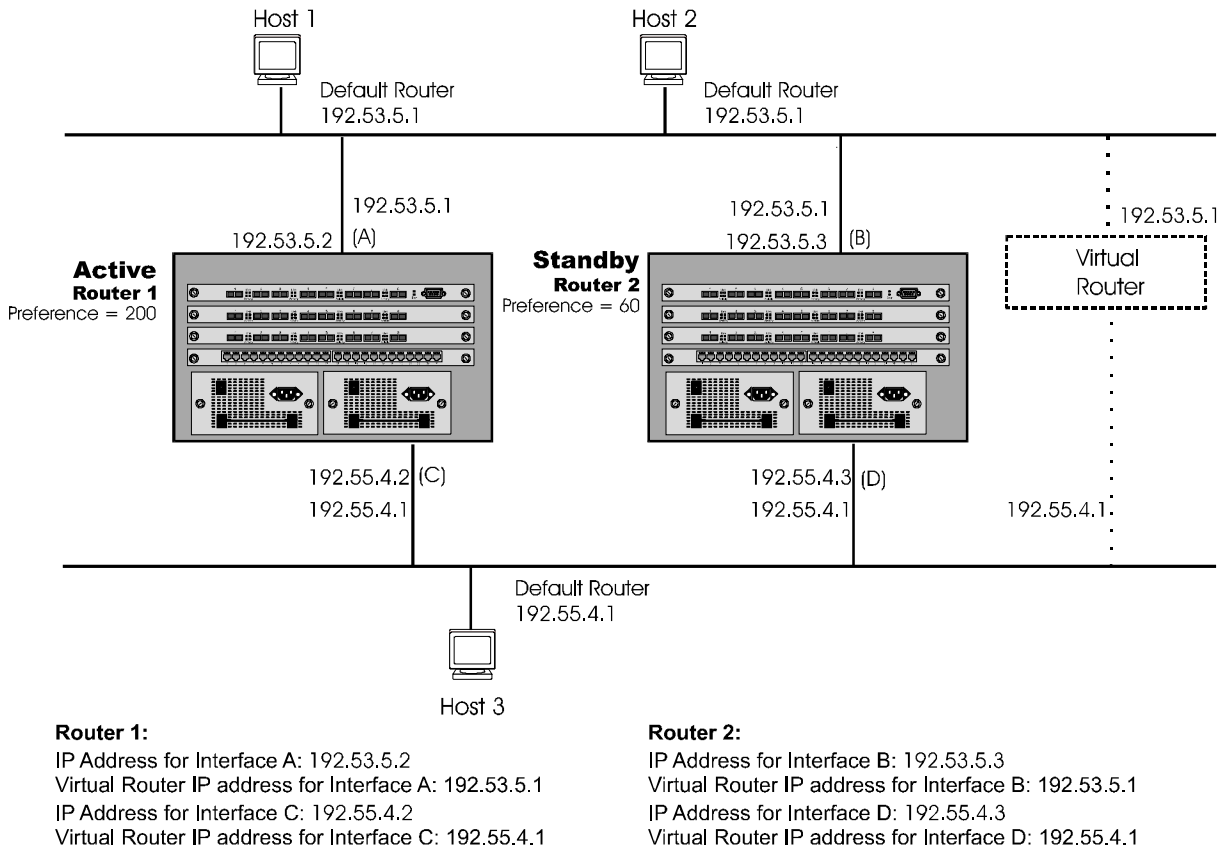
Figure 14.1 SRP operating in an HP 9304M network
