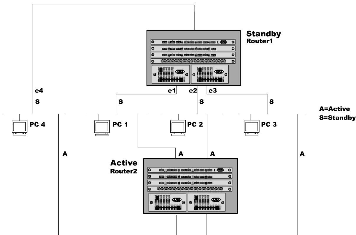
Figure 14.4 Router2 becomes active router after links e1 and e3 fail with multiple track ports defined
