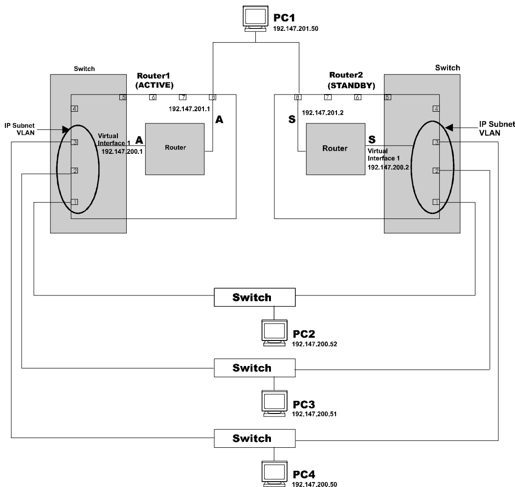
Figure 14.2 Virtual interface as a redundant link
