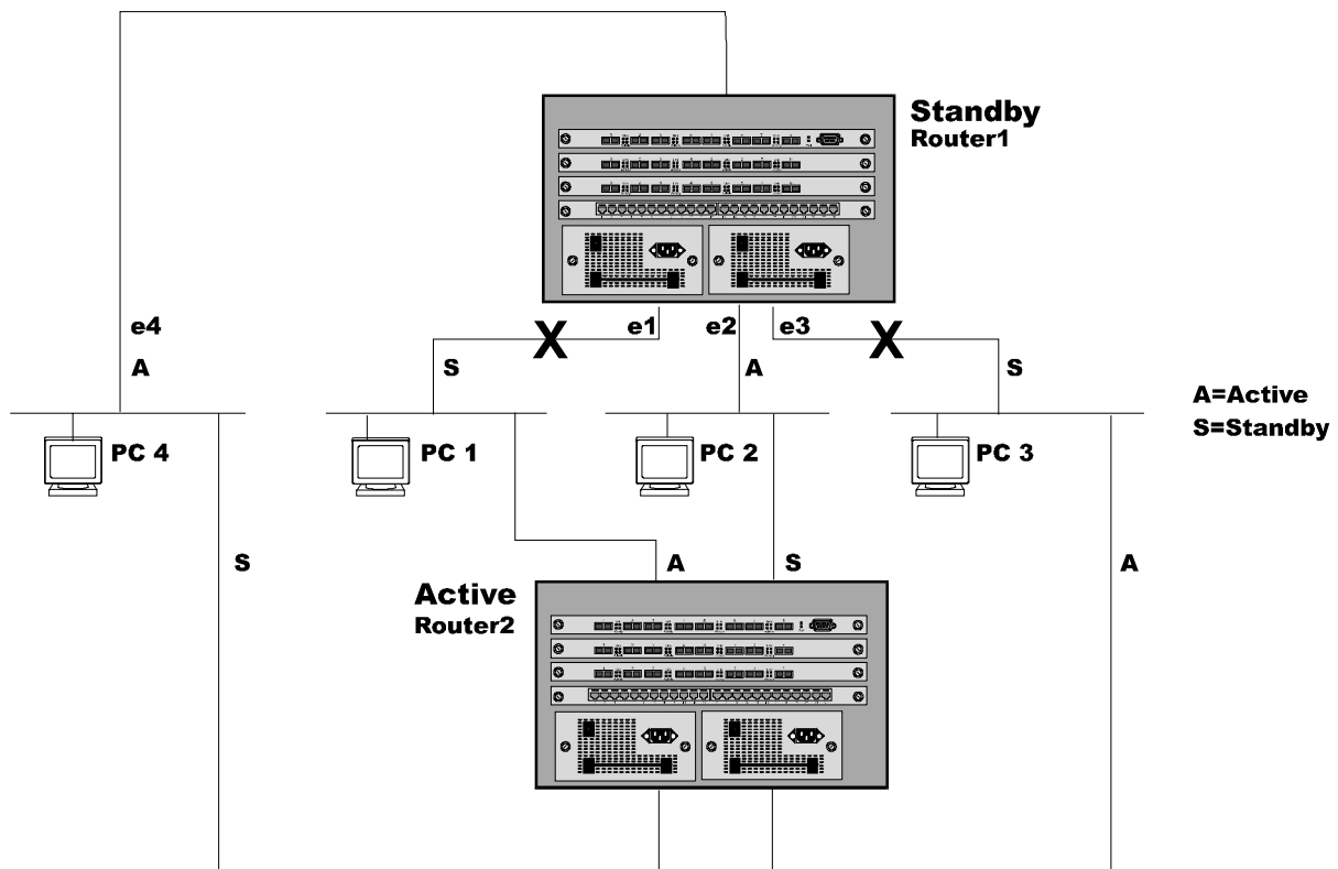
Figure 14.3 Failure of e1 and e3 links results in mixed active and standby links on router1 without the use of multiple track ports
