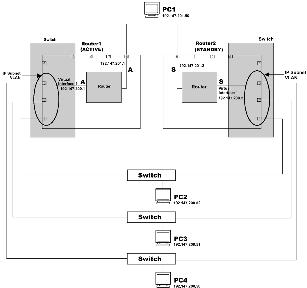
Figure 14.7 Configuring SRP on virtual interfaces
