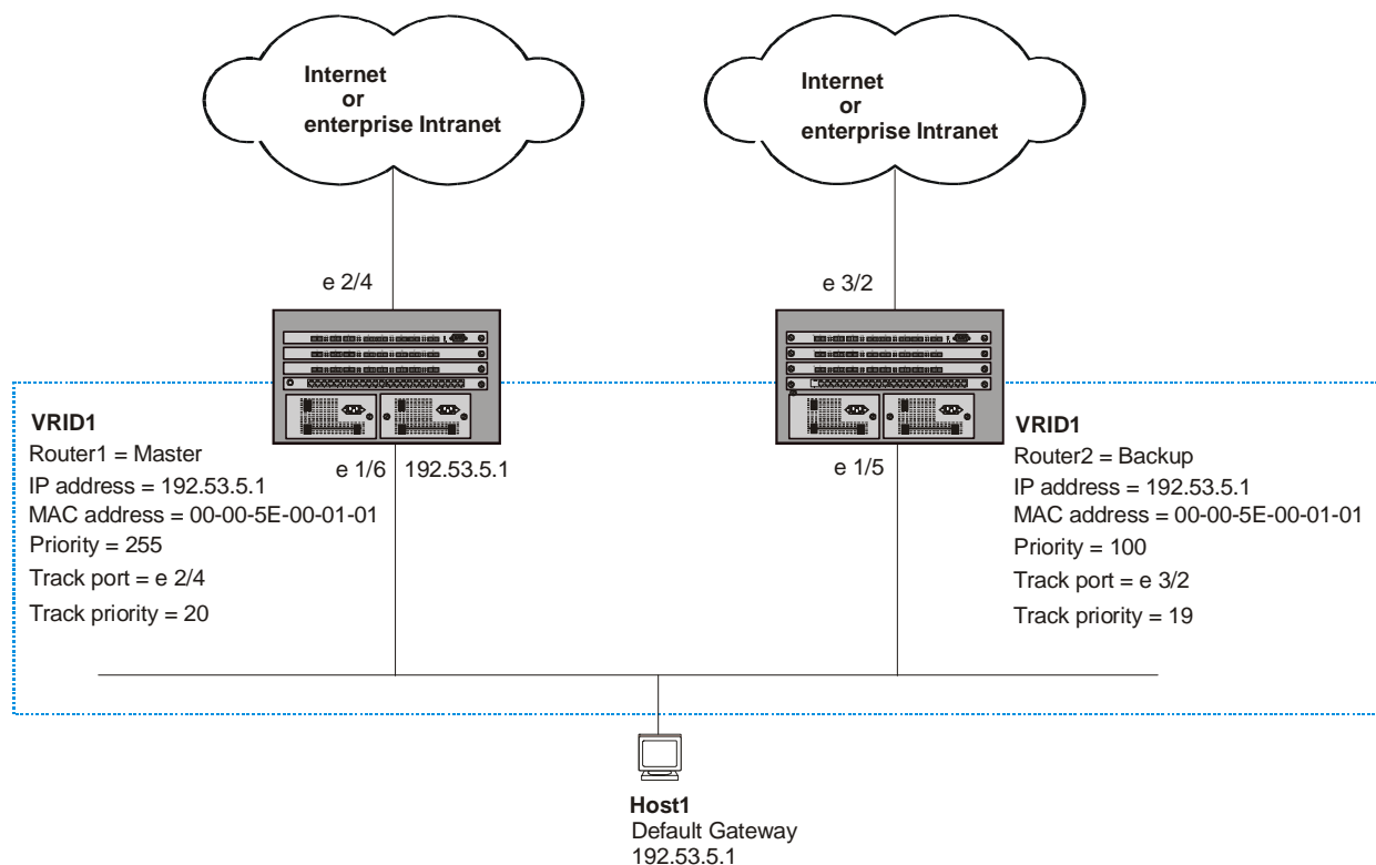
Figure 13.2 Router1 and Router2 are configured as a VRRP virtual router to provide redundant network access for Host1
