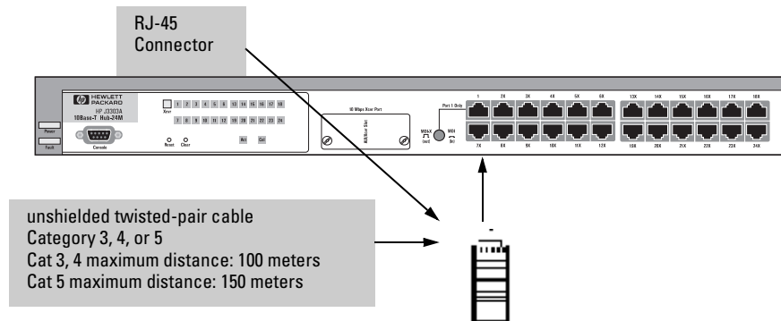
Figure 1-4. The RJ-45 Connector
