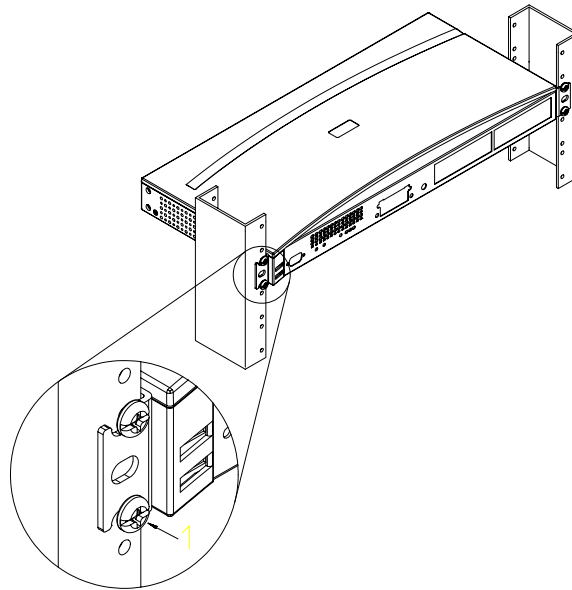
Figure 1-3. Hub-to-Rack Assembly
