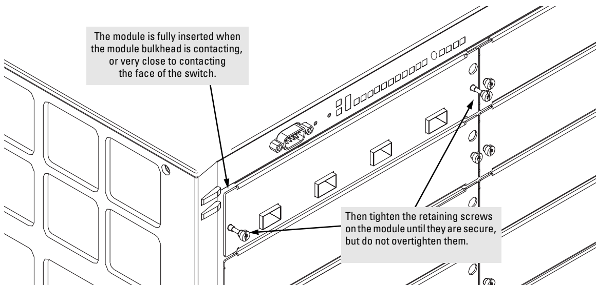
Figure 4. Tighten module retaining screws
