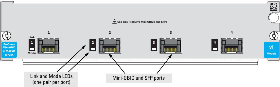
Figure 2. Example: ProCurve Switch Mini-GBIC vl Module
