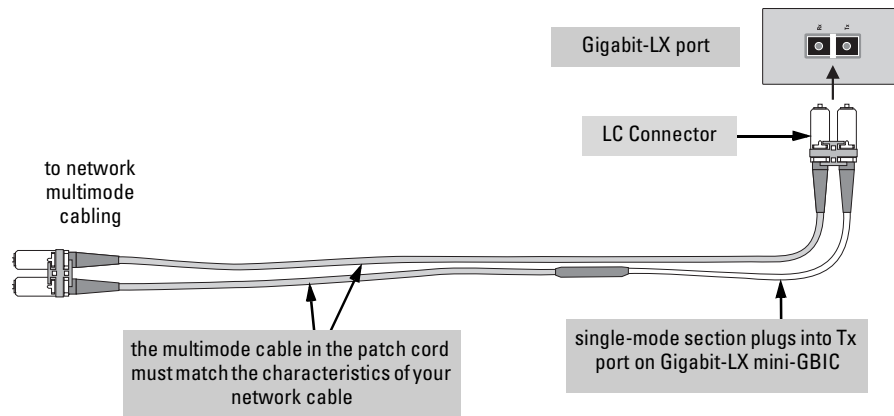
Figure 9. Mode Conditioning Patch Cord
