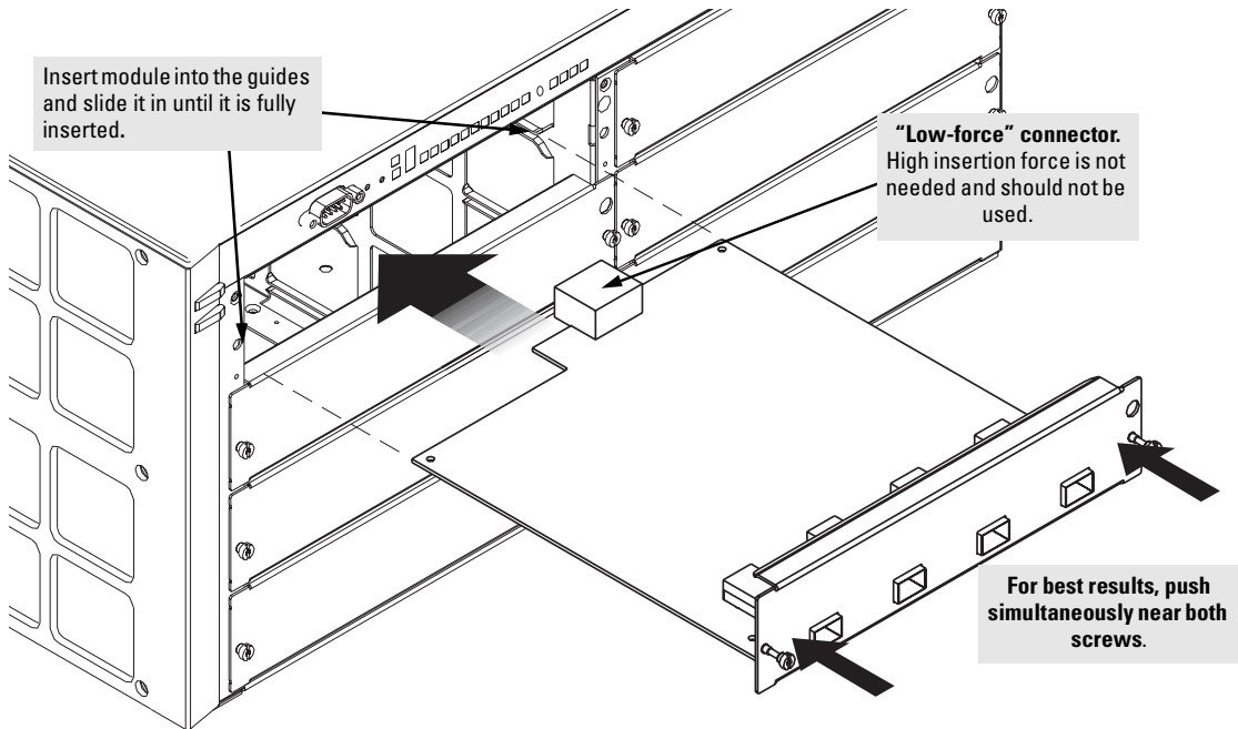
Figure 3. Installing a Module
