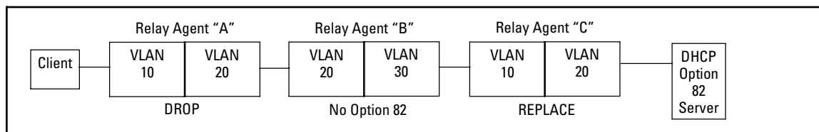
Figure 12. Example Allowing Only an Upstream Relay Agent To Contribute an Option 82 Field
