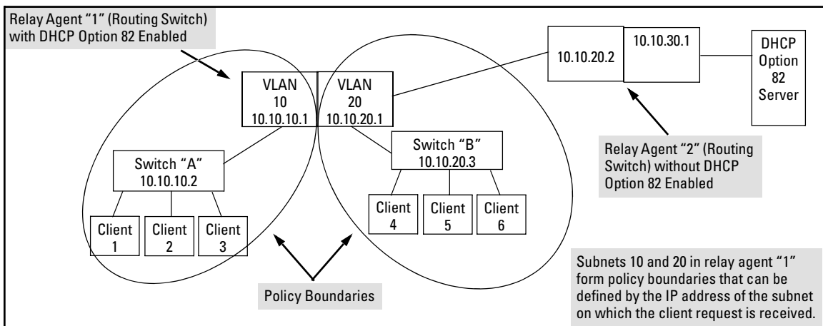
Figure 6. Example of a DHCP Option 82 Application
