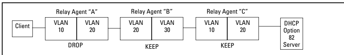
Figure 10. Example Configured To Allow Only the Primary Relay Agent To Contribute an Option 82 Field
