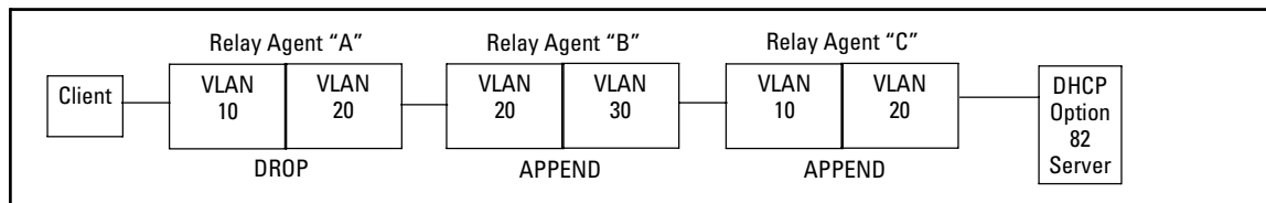
Figure 11. Example Configured To Allow Multiple Relay Agents To Contribute an Option 82 Field
