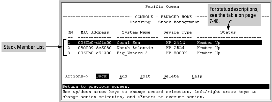
Figure 7-13. Example of Stack Management Screen with Stack Members Listed
